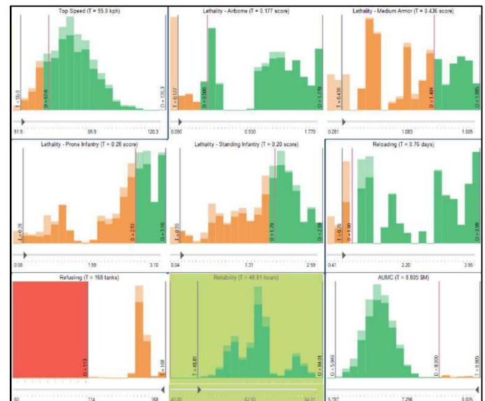
Figure 4: Histograms Showing Distribution of Potential Requirement Values
