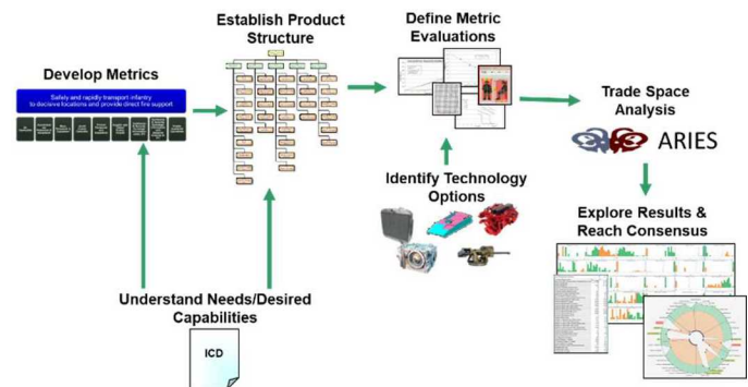
Figure 1: ARIES Methodology
