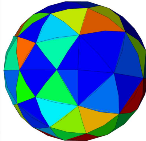
mid-edge nodes on geometry (kinked configuration)
