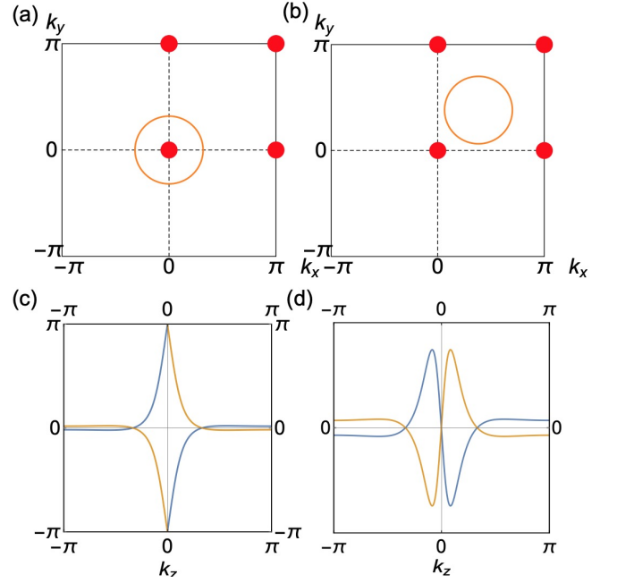
FIG. 6. The Wilson loop eigenvalue flow for the \mathbb{Z}_2 invariant. Panels (a) and (c) show nontrivial \mathbb{Z}_2 invariant, while panels (b) and (d) show trivial \mathbb{Z}_2 -invariant. We construct 2D models starting with a 3D model, and restricting to a 2D surface inside 3D k -space. The 3D model has four Weyl points (red) located at k_z = 0 plane as shown in panels (a) and (b). We choose two different cylinders (topologically, toruses) whose projections are shown as orange loops in panels (a) and (b) for the Wilson loop calculation in panels (c) and (d). Panel (c) shows the flow of Wilson loop eigenvalues when the center of the cylinder lies at (k_x, k_y) = (0, 0) . The cylinder encloses one Weyl point and the invariant is non-trivial. We see one crossing (odd) at \pi and two crossings (even) at 0. Panel (d) shows the flow of Wilson loop eigenvalues when the center of the cylinder lies at (k_x, k_y) = (1.2, 1.2) . The cylinder encloses no Weyl points and the invariant is trivial. We see zero crossing (even) at \pi and three crossings (odd) at 0.
