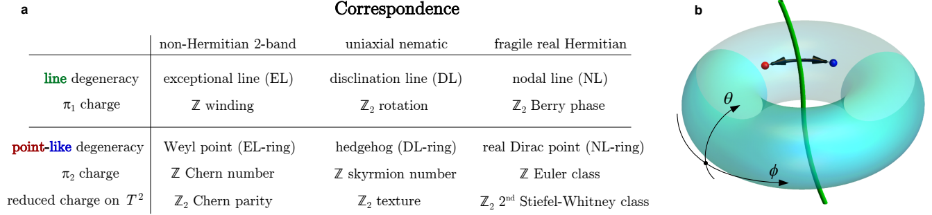
FIG. 5. a) Comparison of the three physical settings discussed in Sec. IV B, IV C, resp. IV D. Although the terminology differs, the description of their singularities (topological defects) is very similar. All three systems exhibit topologically protected line and point defects in 3D, mathematically described respectively by \pi_1 and \pi_2 of the order-parameter space. In each instance, the 1D and 2D invariant interact non-trivially, meaning that the \pi_2 -charge describing a point nodes flips sign if it is carried along a closed path with non-trivial \pi_1 charge. This interaction leads to \mathbb{Z} \rightarrow \mathbb{Z}_2 lowering of the topological invariant on the torus, if there is a non-trivial \pi_1 charge in some direction. b) A 2D torus embedded in 3D, with a green curve indicating an exceptional line, and red and blue points indicating Weyl points of opposite chirality. The two angular coordinates on the torus are denoted \theta and \phi . Since the \phi direction links with the exceptional line, the torus has nontrivial 1D invariant in the \phi direction. By moving one of the Weyl points around the exceptional line, we can change its chirality and obtain a configuration with total charge 2 from this initial configuration of total charge 0; thus total charge 2 represents a topologically trivial configuration, as we understand in terms of braiding Weyl points around an exceptional line.
