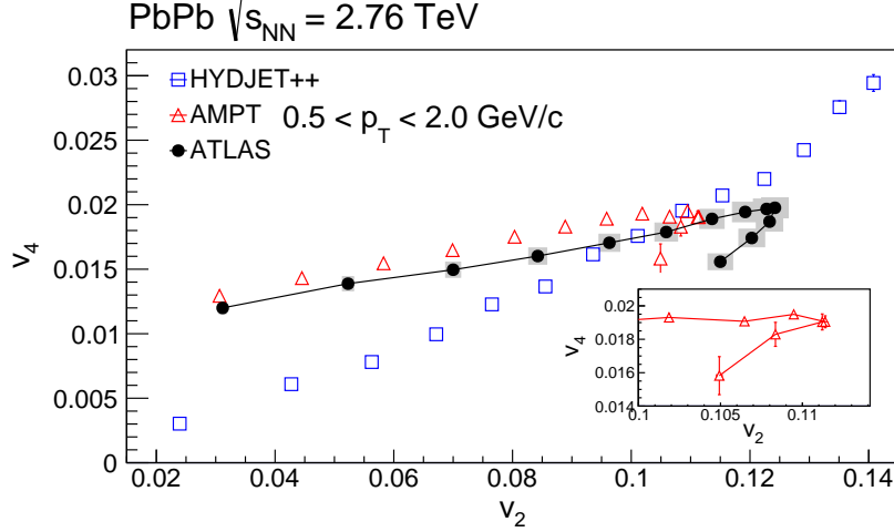
FIG. 3. (Color online) The correlation between v_2 and v_4 from the 0.5 < p_T < 2 GeV/c interval for thirteen (fourteen) 5%-wide centrality classes over the centrality ranges 0–65% (0–70%) in PbPb collisions at 2.76 TeV [34]. The results simulated by the AMPT and HYDJET++ models are shown by the open red triangles and blue squares, respectively. The error bars represent the statistical uncertainties. The shadow boxes represent the systematic uncertainties of the experimental data.
