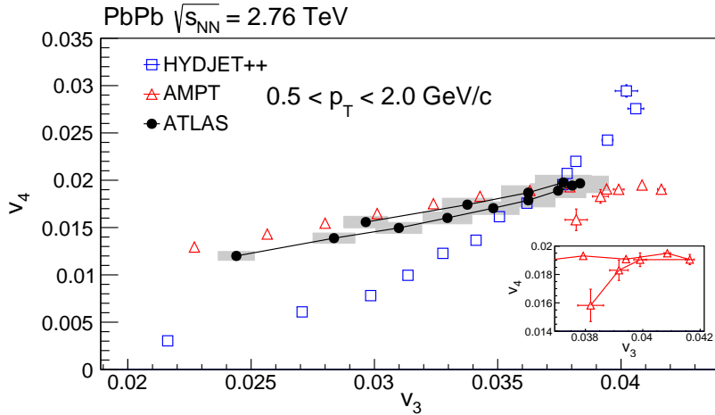
FIG. 4. (Color online) The correlation between v_3 and v_4 from the 0.5 < p_T < 2 GeV/c interval for thirteen (fourteen) 5%-wide centrality classes over the centrality range 0–65% (0–70%) in PbPb collisions at 2.76 TeV [34]. The results simulated by the AMPT and HYDJET++ are shown by the open red triangles and blue squares, respectively. The error bars represent the statistical uncertainties. The shadow boxes represent the systematic uncertainties of the experimental data.
