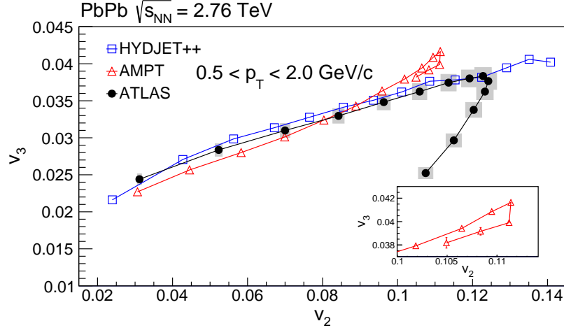
FIG. 2. (Color online) The correlation between v_2 and v_3 from the 0.5 < p_T < 2 GeV/ c interval for fourteen 5%-wide centrality classes over the centrality range 0–70% in PbPb collisions at 2.76 TeV [34]. The results simulated by the AMPT and HYDJET++ models are shown by the open red triangles and blue squares, respectively. The shadow boxes represent the systematic uncertainties of the experimental data, while the statistical uncertainties are smaller than the symbol size.
