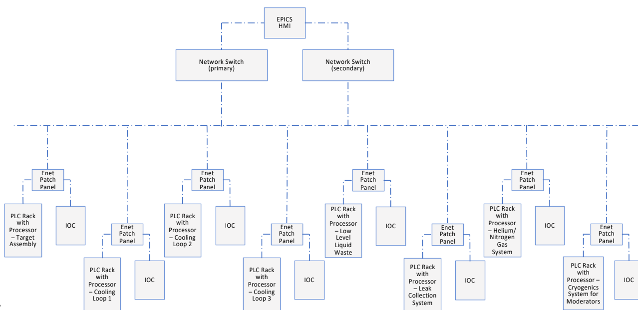
Figure 2: Distributed Control of Target Subsystem for STS.
