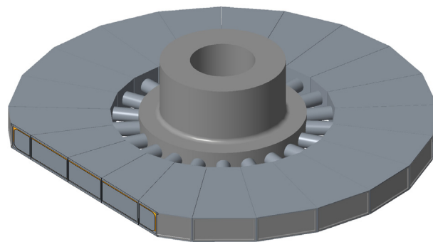
Figure 1: STS Target assembly disk conceptual design, with cutaway to show tantalum cladding on tungsten blocks.
