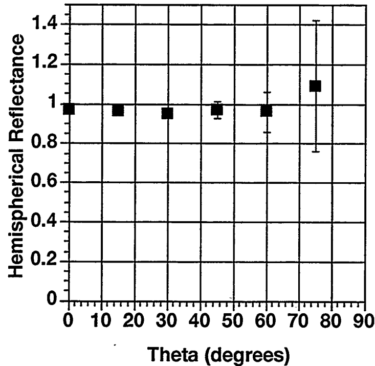
Fig. 4 Measured Hemispherical Reflectance of Spectralon® Calibration Sample. Data measured with the radiometric sensor was used in the determination.
