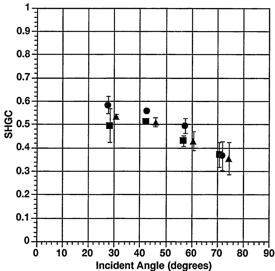
Fig. 8 Angle-Dependent Solar Heat Gain Coefficients for the Venetian Blind Derived from MoWiTT Data. Squares: Oct., 1988 measurement period; triangles: Aug., 1989 measurement period; solid circles: Sept., 1991 measurement period.
