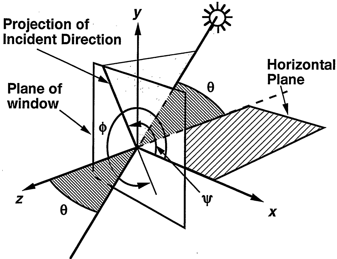
Fig. 9 Relation Between Sun Angles ( \theta, \psi ) and Layer Coordinates ( \theta, \phi ).
