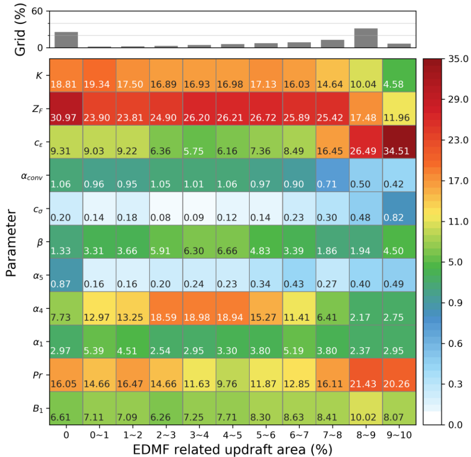
Figure 12. Fraction of the variance of turbine-height wind speed explained by each parameter (colors and numbers in boxes) as a function of EDMF updraft area on 22 August 2016. Box at the top shows the fraction of the domain with that EDMF updraft area.
