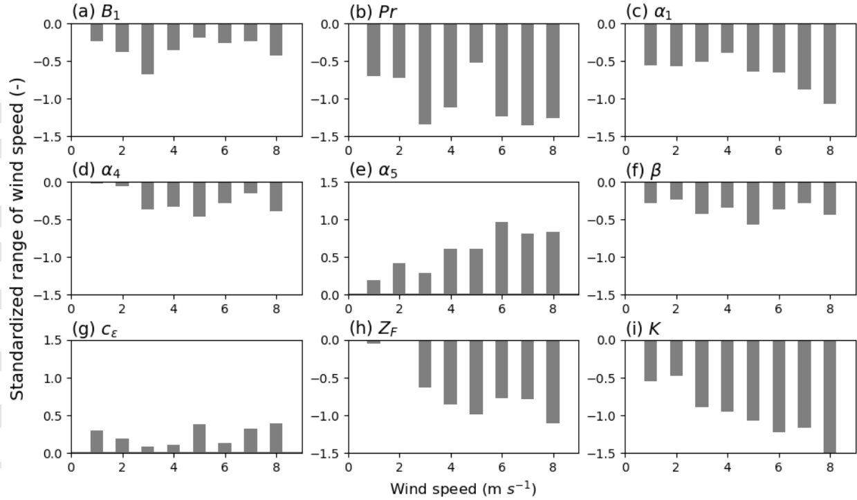
Figure 6. Response (bin 6 – bin 1 differences) of wind speed for the nine most influential parameters over different wind speed ranges for the summer case (Aug 18-24, 2016).
