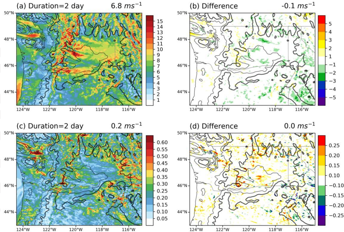
Figure 7. Daily mean wind speed (top) and inter-member standard deviation (bottom; colors) on 22 August 2016 for a simulation duration of 2 days (left) and the difference in wind speed for durations of 2 and 6 days (right). Lines indicate terrain elevations of 500 (thin) and 1000 m (thick).
