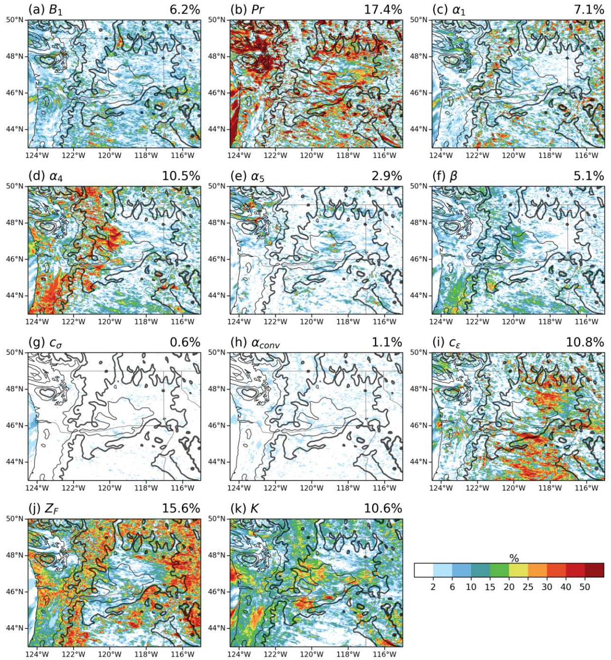
Figure 4. Fraction of the variance of turbine-height wind speed explained by each parameter in Table 1 for 22 August 2016 (simulation of 2-day duration) during daytime. Lines indicate terrain elevations of 500 (thin) and 1000 m (thick). Numbers on the top-right corner of each panel indicate the variance explained by each parameter
