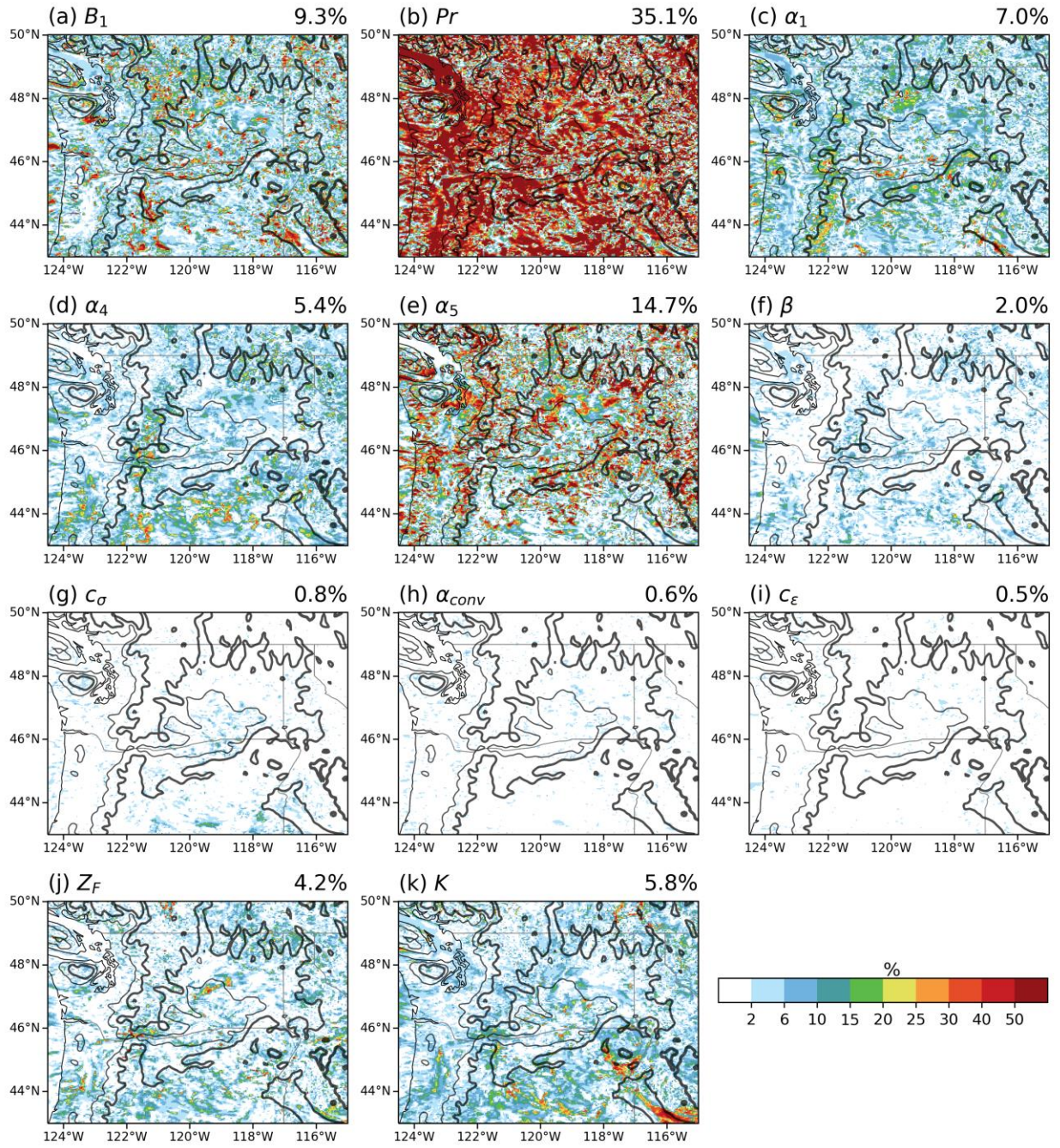
Figure 5. Same as Figure 4 but for 15 January 2017 (simulation of 2-day duration).
