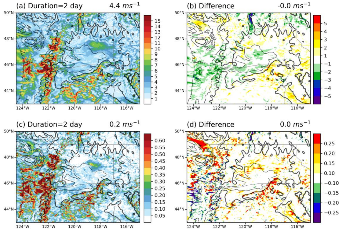
Figure 8. Same as Figure 7 but for 15 January.
