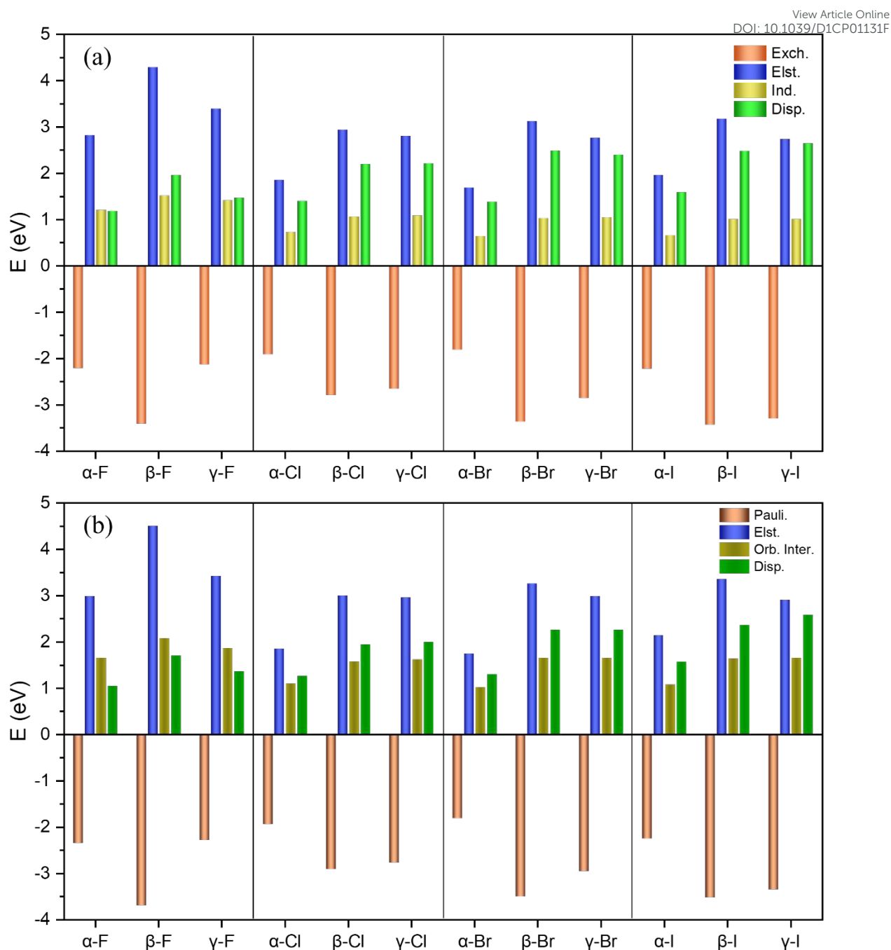
Fig. 5 Components of two different decomposition analysis for CDs·B 12 X 12 2- dianions (X = F-I) (a) exchange, electrostatic, induction and dispersion terms from SAPT analysis at the sSAPT0/jun-cc-pVDZ-(pp) level; and (b) Pauli repulsive, electrostatic, orbital interaction, and dispersion derived from EDA (B3LYP-D3(BJ)/TZ2P) analysis.
