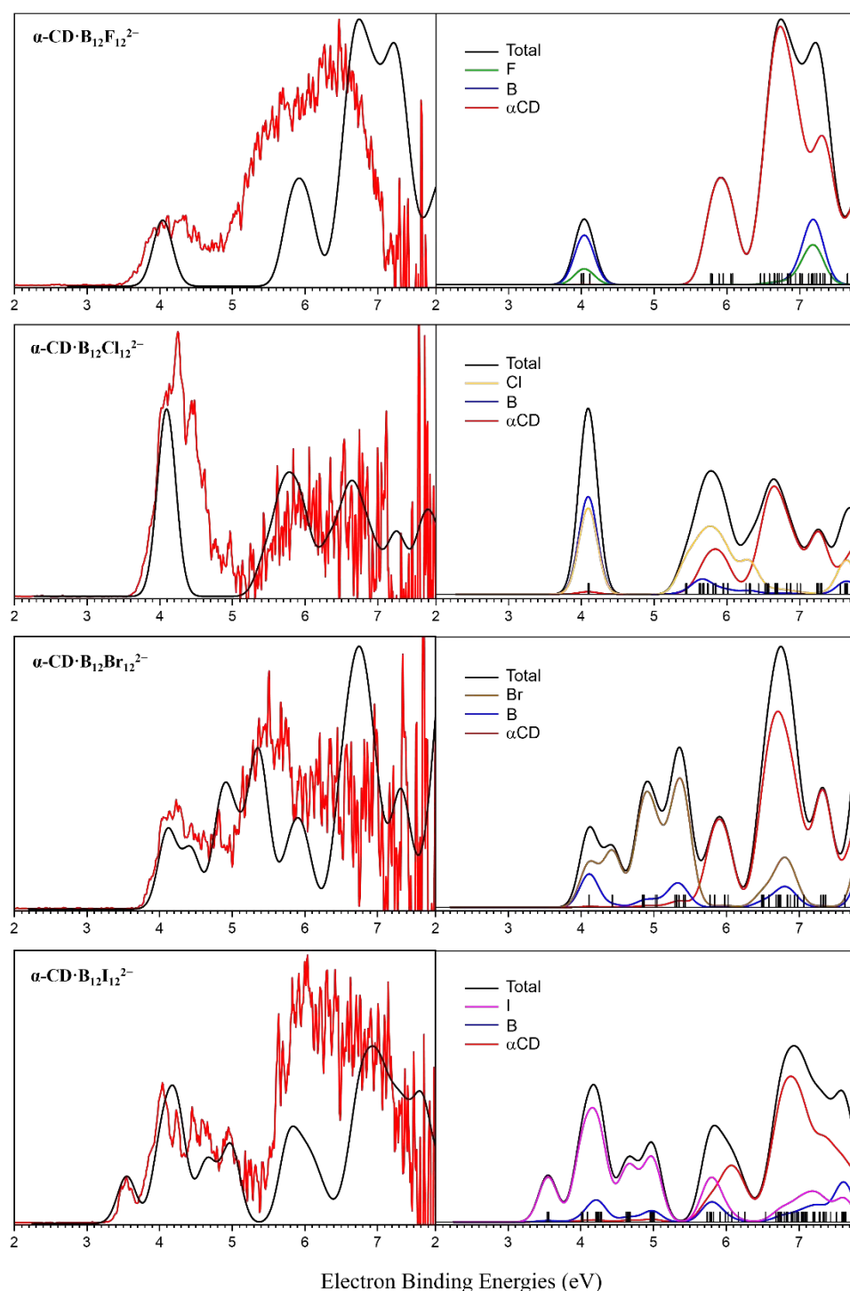
Fig. 4 (Left) Measured (red) and simulated total DOS (black) NIPE spectra of \alpha\text{-CD}\cdot\text{B}_{12}\text{X}_{12}^{2-} (X = F, Cl, Br and I). (Right) Simulated stick spectrum for each complex with the HOMO being shifted to match the experimental VDE. The total DOS and partial DOS (assigned according to the dominant component in specific occupied MOs) spectra were first obtained by
