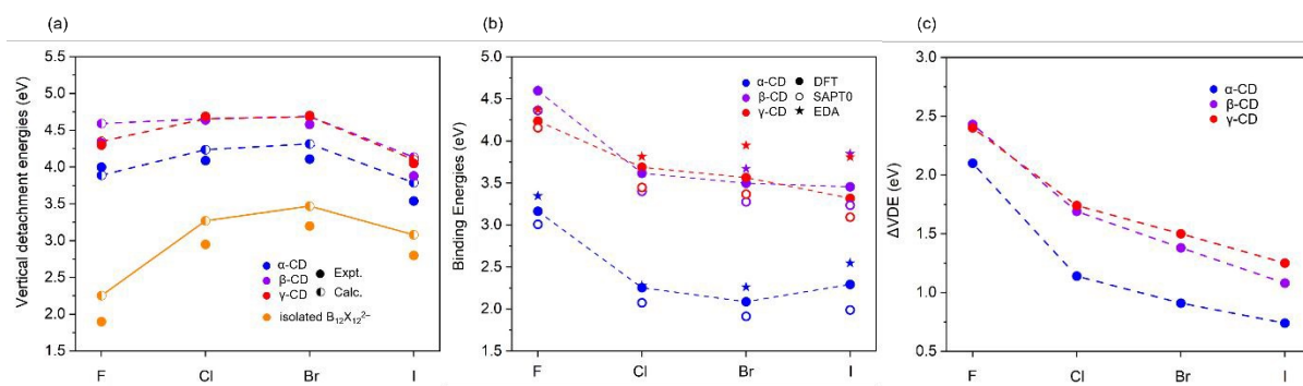
Fig. 2 (a) Experimental (filled circles) and calculated (semi-solid circles) VDEs of isolated \text{B}_{12}\text{X}_{12}^{2-} dodecaborate anions and CDs \cdot\text{B}_{12}\text{X}_{12}^{2-} complexes ( X = \text{F} - \text{I} ); (b) Calculated binding energies of CDs \cdot\text{B}_{12}\text{X}_{12}^{2-} at the levels of M06-2X-D3/ma-TZVP (solid circles), sSAPT0/jun-cc-pVDZ(-pp) (open circles), and B3LYP-D3(BJ)/TZ2P (EDA) (stars); (c) Experimental \Delta\text{VDEs} determined as VDE differences between CDs \cdot\text{B}_{12}\text{X}_{12}^{2-} and the corresponding isolated \text{B}_{12}\text{X}_{12}^{2-} .
