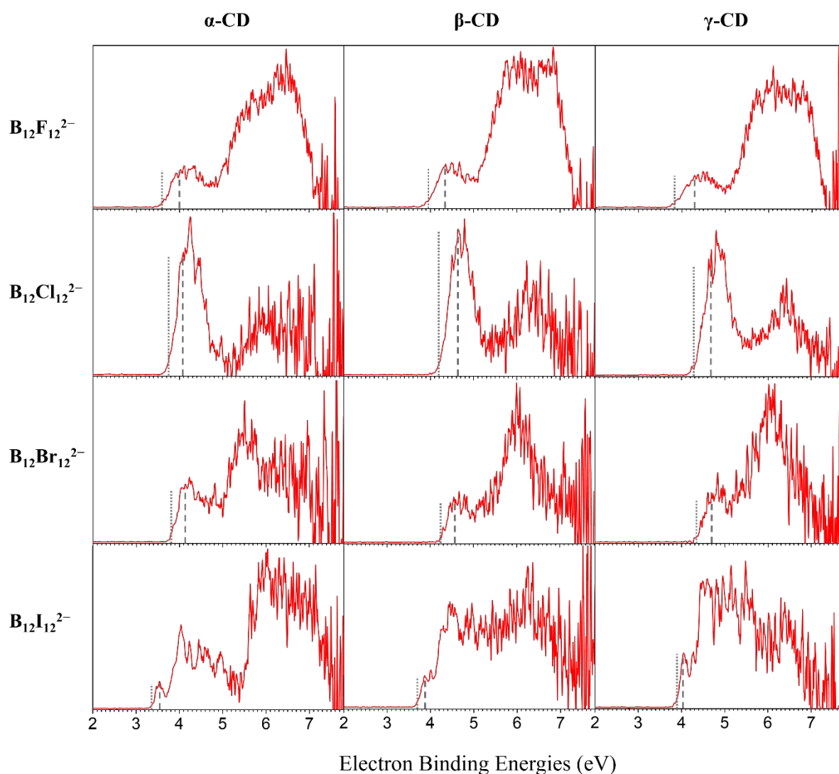
Fig. 1 The 20K NIPE spectra of \chi\text{CD} \cdot \text{B}_{12}\text{X}_{12}^{2-} ( \chi = \alpha-, \beta-, \gamma-; X = F, Cl, Br, and I) measured with 157 nm photons. The measured spectra for the X=F series are adapted from reference 22 . The gray dotted and dashed lines designate the spectral EBE positions from which the ADEs and VDEs are determined, respectively.
