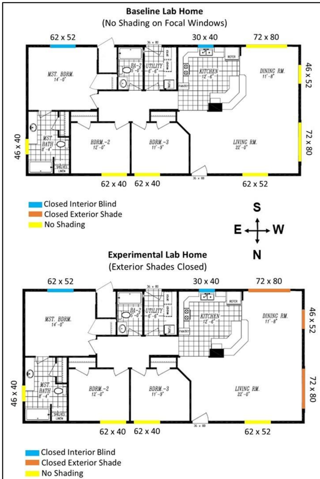
Figure 8. Lab Home Configurations for Test Cases 2 and 3
