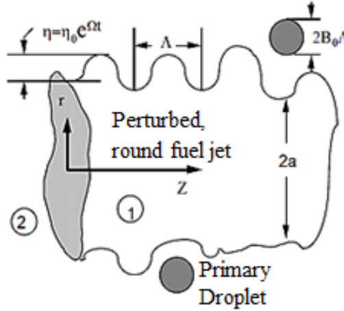
Figure 1.7: Schematic depicting primary breakup of a liquid fuel jet due to the aerodynamic growth of waves, modified from [16].
