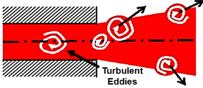
Figure 1.17: Schematic of turbulence primary breakup model, modified from [43]. Turbulent fluctuations formed within the injector create disturbances at the liquid-gas interface, which grow and result in the formation of primary droplets
