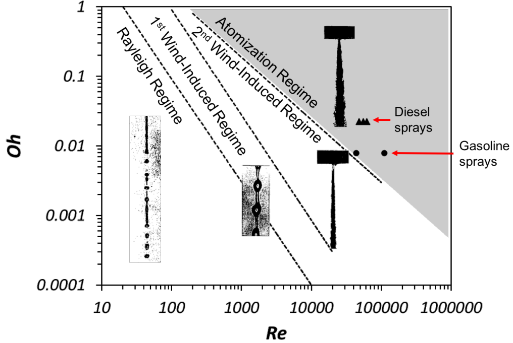
Figure 1.6: Four main regimes of round jet breakup (adapted from [16]), namely the Rayleigh regime, the first wind-induced regime, the second wind-induced regime, and the atomization regime. Fuel sprays are characterized by high Re_f and therefore typically reside within the atomization regime.
