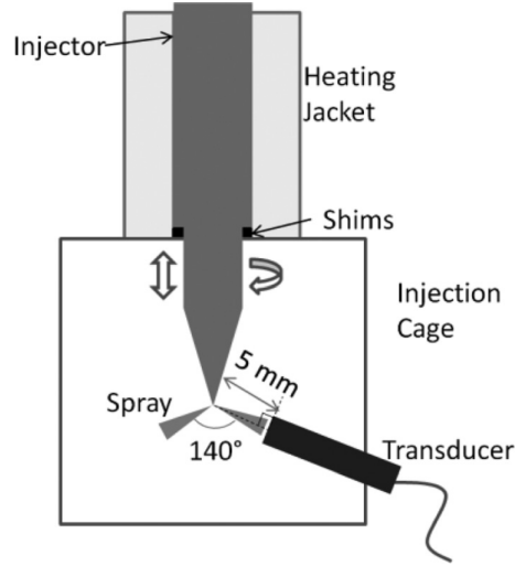
Figure 2.11: Schematic of apparatus for rate-of-momentum measurement [122]. The schematic is shown for a multi-hole injector.
