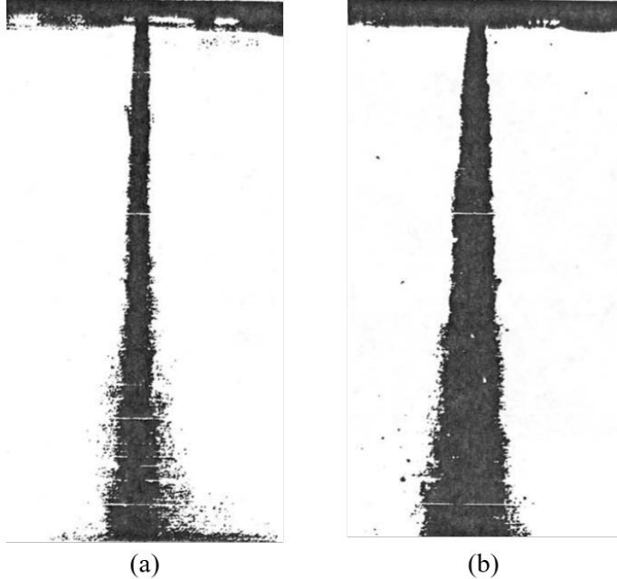
Figure 1.8: Sample images of sprays from the seminal work by Reitz [30], detailing the influence of turbulent flow development within the nozzle on the general spray characteristics. A nozzle with fully-developed turbulent flow ( L/d_j = 85 ) is shown in (a) while a nozzle with flow transitioning from laminar to turbulent ( L/d_j = 10.1 ) is shown in (b)
