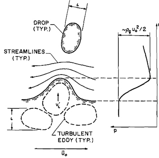
Figure 1.13: Schematic of aerodynamically enhanced turbulence breakup, modified from [19]. The size of droplets formed are proportional to the size of the turbulent eddies, l_i .
