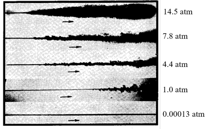
Figure 1.11: Photographs detailing the effect of ambient pressure on fuel jet breakup, modified from Lee and Spencer 1.11.
