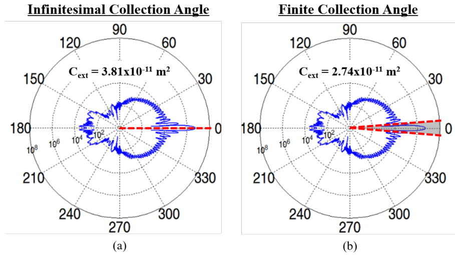
Figure 3.1: Influence of collection angle on collection of forward scattered light and \overline{C_{ext}} from a 5\mu\text{m} droplet. \theta_{1/2} \approx 0^\circ is shown in (a) while \theta_{1/2} = 5.6^\circ is shown in (b).
