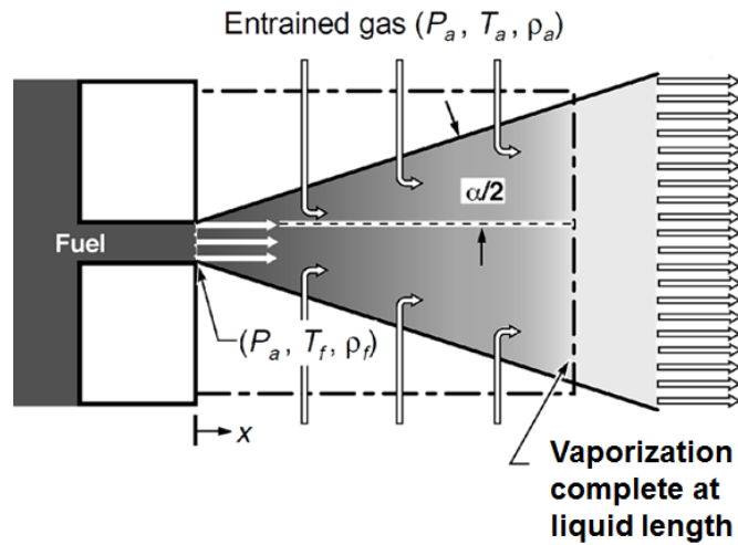
Figure 1.2: Schematic of Sieber's dense gas jet model, modified from [7] to represent the scaling of liquid length.
