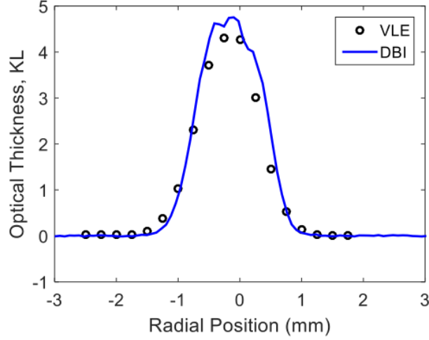
Figure 7.1: Comparison between VLE and DBI extinction of Spray A (150 MPa, 22.8 kg/m 3 ) at an axial location of 7.5 mm from the injector tip. Overlap of data indicates consistent measurements.
