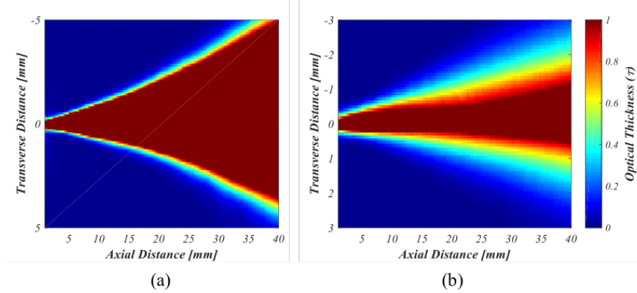
Figure 2.10: Example 2D extinction map obtained from DBI measurements are shown for P_{inj} of 50 MPa and P_{amb} of (a) 2 MPa and (b) 0.1 MPa.
