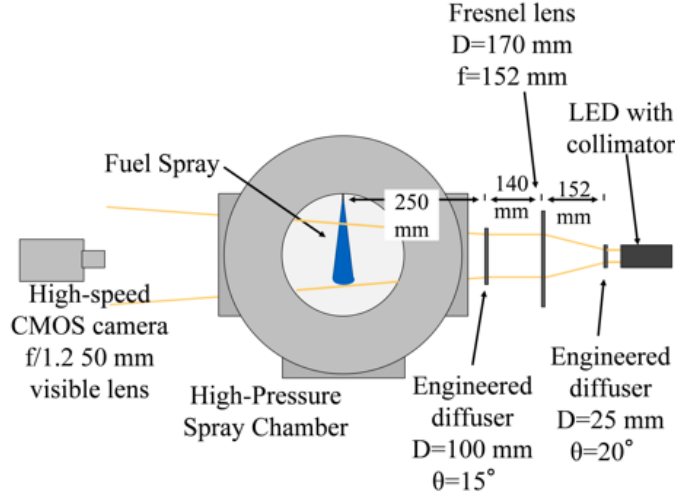
Figure 2.9: Experimental arrangement for diffused back-illuminated imaging, based on the recommendations outlined by Westlye and co-workers [129].
