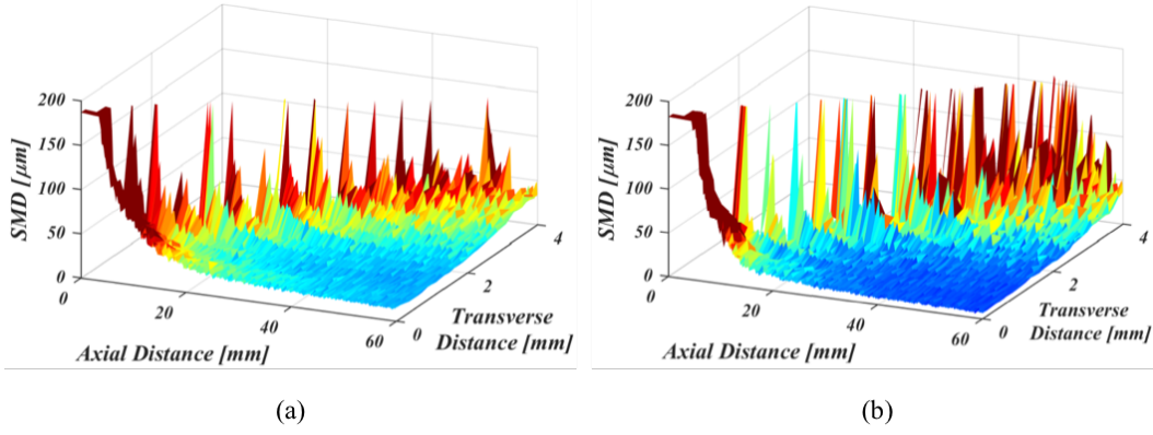
Figure 5.6: Sample 2-D time-averaged SMD map as predicted by the KH-ACT model for the Spray D nozzle at ambient and injection conditions of (a) \rho_f/\rho_g = 310 , P_{inj} = 50 MPa and (b) \rho_f/\rho_g = 310 , P_{inj} = 150 MPa. Only half of the spray is shown in order to clearly illustrate the difference in predicted SMD between the central and peripheral regions of the spray.
