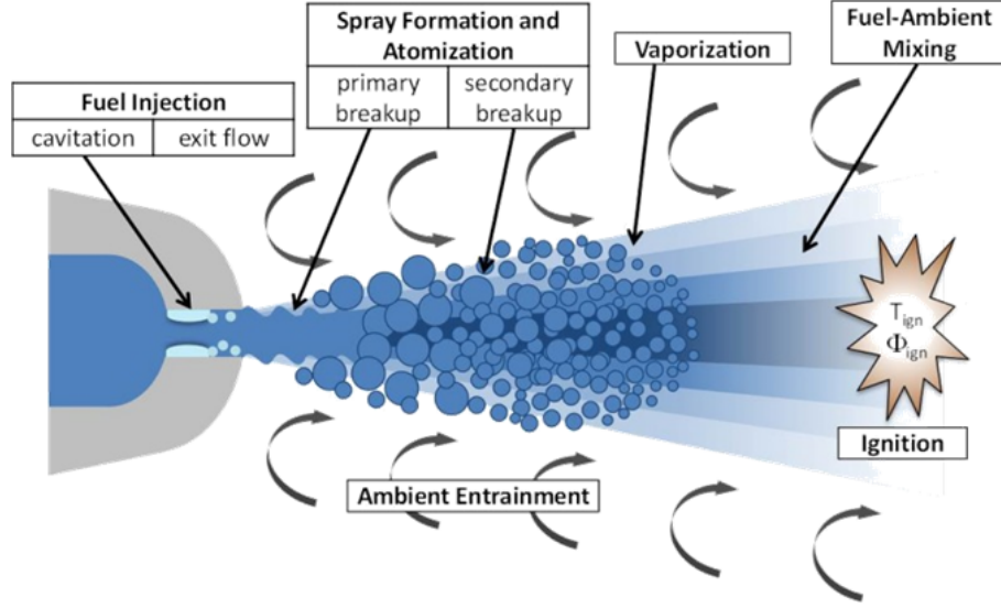
Figure 1.5: Physical processes influencing fuel spray development in a direct injection engine-relevant environment [20].
