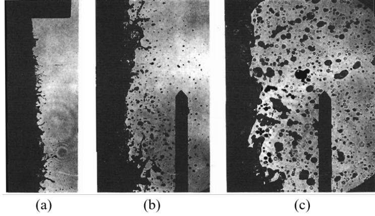
Figure 1.12: Pulsed shadowgraphs near the liquid-gas interface of a low-velocity water jet [50] (a) at the nozzle exit and at distances of (b) 10 and (c) 50 nozzle diameters from the nozzle exit.
