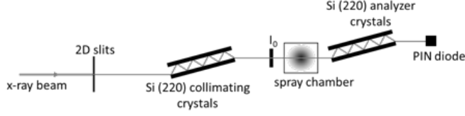
Figure 2.4: A schematic of the Ultra-Small Angle X-ray Scattering experiment [94].
