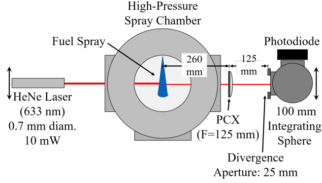
Figure 2.7: A schematic of the high pressure spray chamber and laser extinction measurement set-up.
