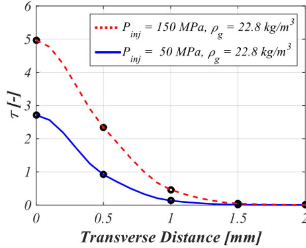
Figure 2.8: Comparison of radial distribution of laser extinction measurements, \tau , at two different injection pressures (50 and 150 MPa) [86]. The distributions are shown for a location 8 mm from the injector nozzle exit. Each experimental data point shows the mean optical thickness, ensemble-averaged over 30 injections.
