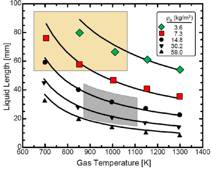
Figure 1.3: Comparison of Sieber's dense gas jet model predictions with diesel spray liquid length measurements, modified from [7].
