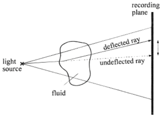
Figure 1.15: Schematic of shadowgraph imaging technique without optical components [57].
