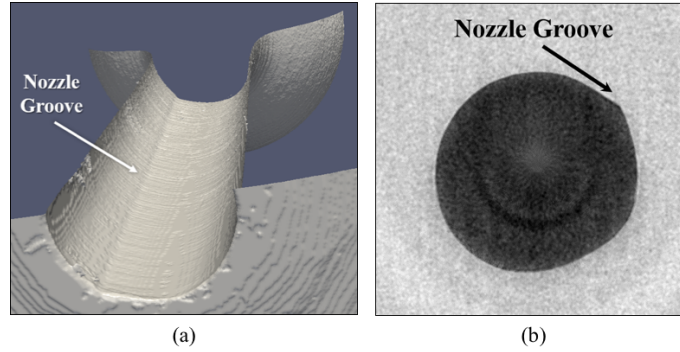
Figure 2.2: Detailed internal nozzle geometry measurements from x-ray tomography conducted at the APS [94]. Renderings for the constructed (a) iso-surface of Spray D #209133 and (b) nozzle hole are shown.
