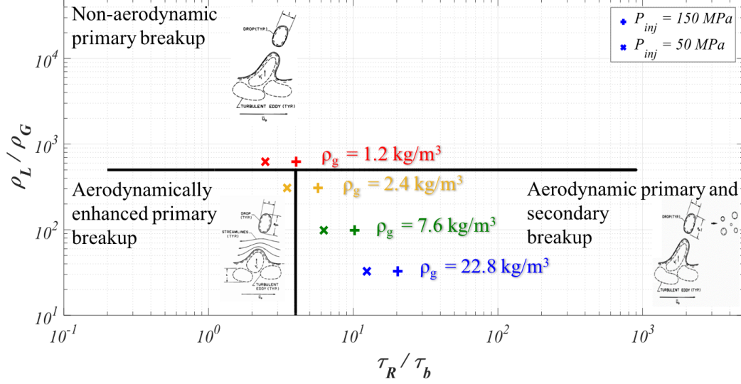
Figure 1.14: Turbulent primary breakup regime map, adapted from the work of Faeth and co-workers [19].
