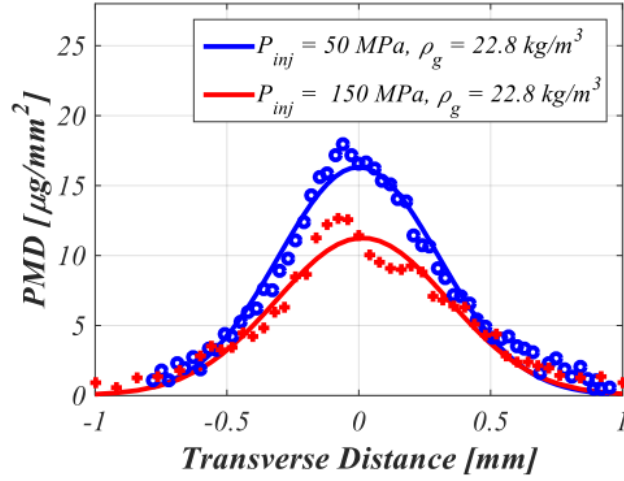
Figure 2.3: Comparison of radial distribution of x-ray radiography measurements, at an axial distance of 8 mm from the nozzle exit [1].
