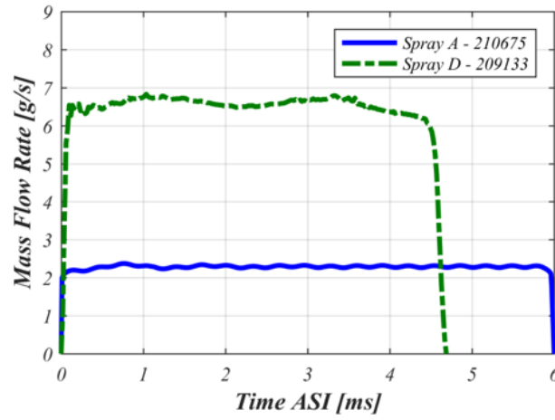
Figure 2.12: Comparison of the modeled ECN Spray A ROI [114, 131] and measured Spray D ROI [88] profiles at \rho_g = 22.8 \text{ kg/m}^3 and P_{inj} = 50 \text{ MPa} .
