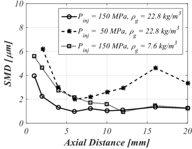
Figure 2.5: Comparison of axial distributions of USAXS SMD measurements along the spray centerline [1]. Data is shown for a range of ambient density and injection pressure conditions for the ECN Spray A injector.
