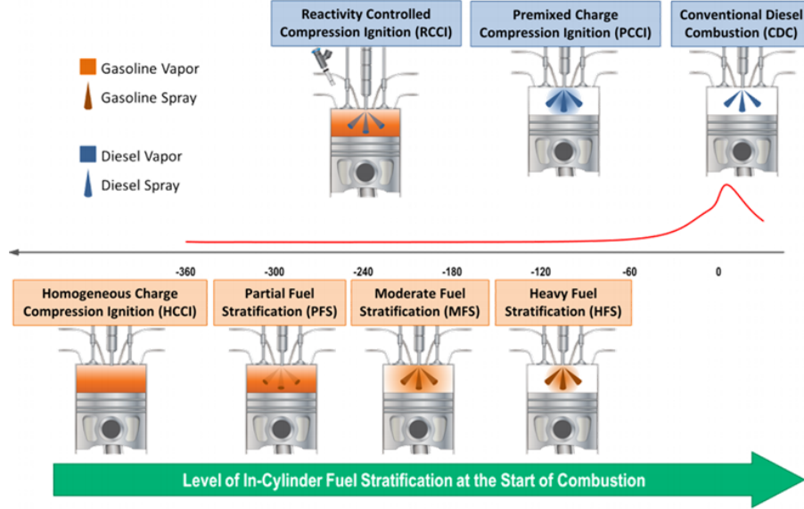
Figure 1.1: Range of advanced compression ignition combustion strategies using gasoline and/or diesel fuel to achieve low temperature combustion [6]. Combustion strategies are ordered according to their respective fuel injection timing with respect to top dead center (0 CAD).
