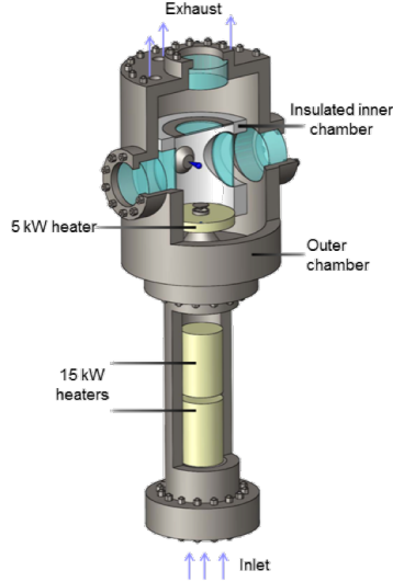
Figure 2.6: An illustration of the continuous flow optically-accessible spray chamber.
