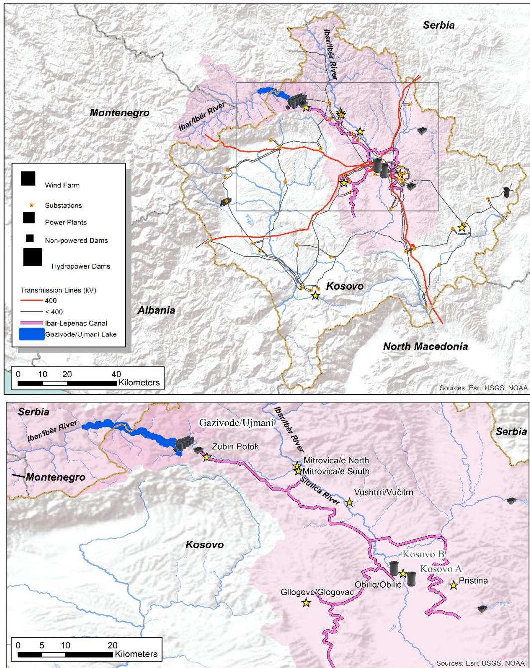
Figure 1. Kosovo water and electricity infrastructure. The inset represents the Gazivode/Ujmani hydosystem that supplies the cities of Mitrovica/ë North and Mitrovicë/a South, Vushtri/Vučitrn, Obiliq/Obilić, Glogovc/Glogovac, and Pristina with freshwater through the Ibër-Lepenc/Ibar-Lepenac Canal. The colored area represents the Ibar/Ibër River basin area draining into Kosovo, and within Kosovo, before flowing into Serbia. (Map Credit: Jerry Tagestad and Corrine DeCiampa – PNNL. Data Credits: Data were digitized on screen from resources at https://kostt.com and http://www.iber-lepenc.org ; Background map ESRI 2021.)
