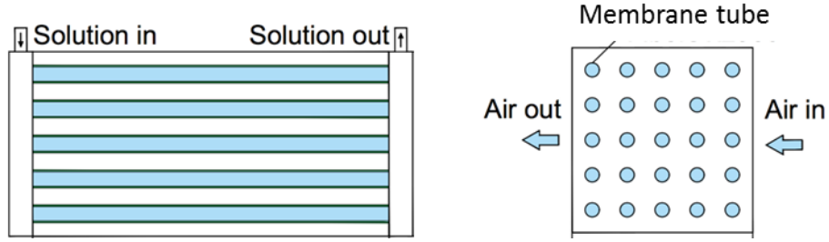
Figure 3. Concept design of a MILDAD using membrane tubes: a side view (left) and a section view (right).
