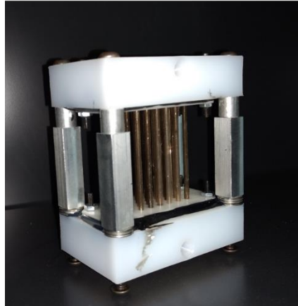
Figure 4. A small-scale prototype of the MILDAD built by Xergy Inc.
