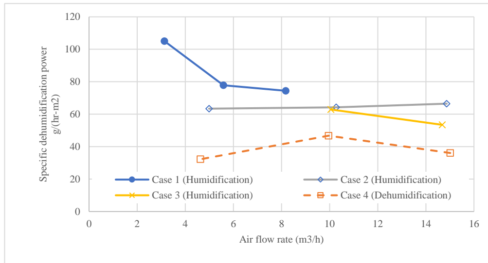
Figure 6. Measured specific vapor transportation rate of the small-scale MILDAD prototype in dehumidification and humidification operation at various airflow rates.
