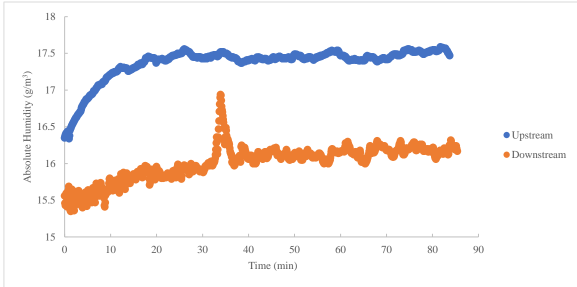
Figure 8: Dehumidification performance of dehumidifier module at 0.28 m 3 /min. *Note that the spike in AH between 30 and 40 min was caused by a leak in the system. This leak was resolved during the test and these data points were disregarded in the analysis.
