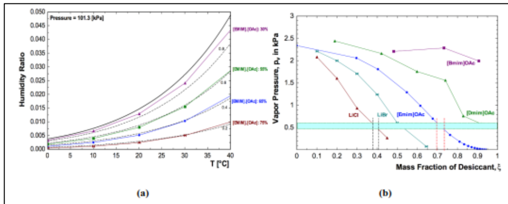
Figure 1: Properties of [EMIM][OAc] (a) dehumidification capacities at different concentrations, (b) commonly used concentration ranges of different desiccants
