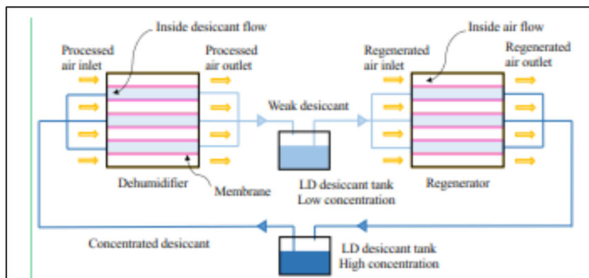
Figure 2: Schematic diagram of basic procedure of membrane-based liquid desiccant system
