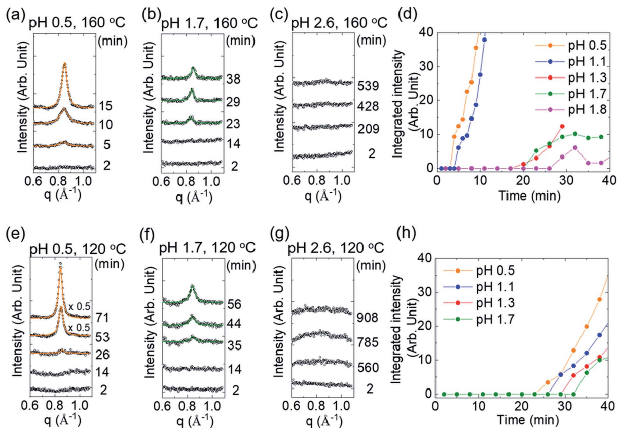
Fig. 2 Evolution of the \delta' -MnO 2 (200) peak and onset of crystallization. The \delta' -MnO 2 (200) peak evolution at representative pH and time points at 160 °C (a–c) and 120 °C (e–g), showing the onset point and intensity growth after. The experimental data and the fits are shown by the open circles and solid lines, respectively. The onset of \delta' -MnO 2 is defined as the time point that the (200) peak shape can be meaningfully fitted by a Lorentzian function. The integrated intensity of the (200) scattering peak in the first 40 min of the hydrothermal reaction at 160 °C (d) and 120 °C (h). For the data after 40 min and not presented here in the manuscript, please see Fig. S2 in ESI 3.†
