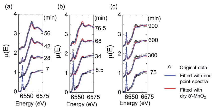
Fig. 4 Linear combination fitting results of the Mn K edge spectra. Representative fitting results for (a) pH 0.5, (b) pH 1.1, and (c) pH 2.6, showing the experimental data (open circles), fit with the reference dry \delta' - \text{MnO}_2 powder (red line), and fit with endpoint scans of each of the reactions (blue line). For pH 2.6, due to the fact that the edge did not reach the \delta' - \text{MnO}_2 endpoint, the 85 min spectrum in pH 1.1 was used as an endpoint instead.
