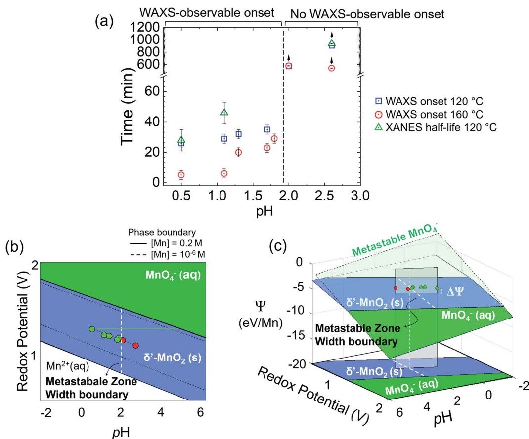
Fig. 6 Trend of MnO_2 onset time and the metastable zone width. (a) A summary of the \delta' - MnO_2 onset time and Mn_{tet} half-life as a function of pH and reaction temperature, measured using WAXS and XANES, respectively. The datapoints with upward arrows represent the absence of \delta' - MnO_2 onset when the in situ WAXS observation ended. (b) The boundary of metastable zone width (white dashed line) marked on a section of the Mn Pourbaix diagram including the MnO_4^- (aq) and \delta' - MnO_2 phases (see Fig. S7 in ESI 9 for the full diagram). The Pourbaix diagram is shown at the experimental Mn concentration of 0.2 M. A comparison of the phase boundary at [Mn] = 10^{-6} M is shown in black dashed lines. The green dots show the experimental conditions where crystallization is observed, and the red dots represent conditions where nucleation is not observed even after 9 hours. (c) Diagram showing the Pourbaix free-energy landscape above Fig. 6(b), illustrating the electrochemical supersaturation ( \Delta\Psi ) of MnO_4^- (aq) relative to \delta' - MnO_2 . The thermodynamic driving force ( \Delta\Psi ) does not change significantly in the vicinity of pH 2, implying that the thermodynamic effect is not the main cause of the induction time difference.
