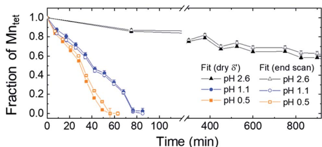
Fig. 5 Atomic fraction Mn_{tet} along with reaction time. Atomic fraction as a function of reaction time is obtained from linear combination fitting of the Mn K edge spectra. Filled and open symbols represent results obtained by using dry \delta' - MnO_2 power and endpoint scans, respectively.
