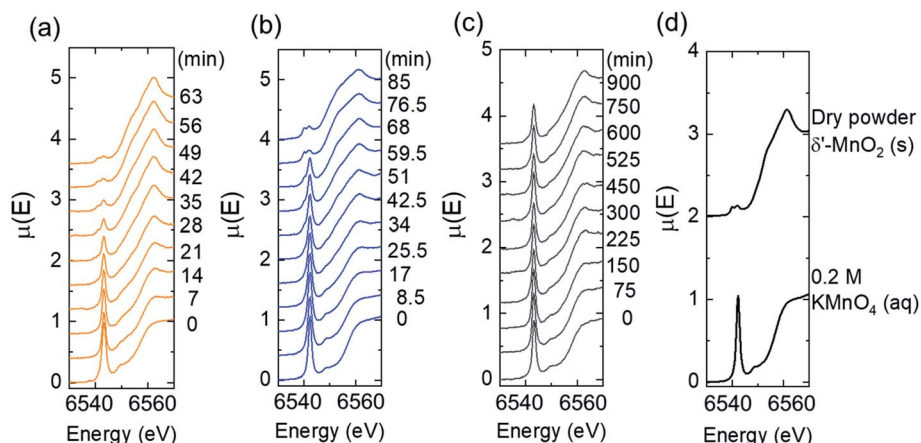
Fig. 3 Mn K edge spectra evolution at varying pH. (a–c) The Mn K edge of (a) pH 0.5 (b) pH 1.1, and (c) pH 2.6 at 120 °C as a function of reaction time. The data labeled 0 min represent the spectra acquired at room temperature before starting the hydrothermal reaction. (d) Reference spectra of 0.2 M \text{KMnO}_4 water solution ( \text{Mn}_{\text{tet}} ) and dry \delta' - \text{MnO}_2 powder ( \text{Mn}_{\text{oct}} ).
