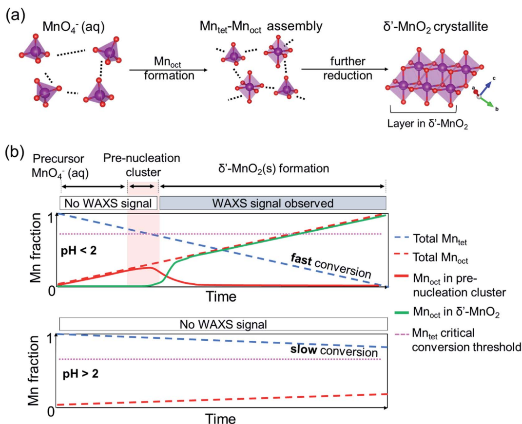
Fig. 7 Hypothetical mechanism of \delta' - \text{MnO}_2 formation at the early stages. (a) Individual \text{MnO}_4^- ions in the solution agglomerate, forming a pre-nucleation assembly consisting of \text{Mn}_{\text{tet}} and \text{Mn}_{\text{oct}} . Upon further reduction, edge-sharing \text{MnO}_6 octahedra form, eventually transforming to solid \delta' - \text{MnO}_2 . (b) A schematic of the development of \delta' - \text{MnO}_2 along with the atomic fraction of \text{MnO}_4^- ( \text{Mn}_{\text{tet}} ) and \text{MnO}_6 ( \text{Mn}_{\text{oct}} ) during the hydrothermal synthesis. The linearly decreased \text{Mn}_{\text{tet/oct}} fraction in the solution is corresponding to the XANES data shown in Fig. 5. As the concentration of the \text{Mn}_{\text{tet}}-\text{Mn}_{\text{oct}} pre-nucleation assembly passes the critical conversion threshold, the nucleation of \text{MnO}_2 solid begins. In the case of \text{pH} > 2 , the conversion of \text{Mn}_{\text{tet}} to \text{Mn}_{\text{oct}} is too slow, therefore the critical conversion threshold cannot be reached within an observable time frame. This schematic demonstration is adapted from previous works of Smeets et al. 50 and Gebauer et al. 51
