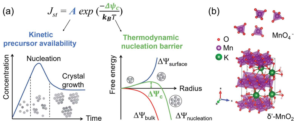
Fig. 1 Schematics showing the factors controlling the steady-state nucleation rate and atomic structures of the Mn-species discussed in this work. (a) The two major factors, precursor availability and nucleation barrier, controlling the kinetic and thermodynamic aspects of steady-state nucleation rate ( J_{st} ), respectively. 34,35 (left) The precursor availability can be interpreted as the abundance of solute supply for nucleation to happen. The LaMer nucleation model describes the correlation between precursor concentration (represented by the gray balls) as a function of time. (right) The nucleation barrier ( \Delta\Psi_c ), defines the minimum radius that allows a nuclei to be stable. \Delta\Psi_c originates from the competition between bulk free energy ( \Delta\Psi_{\text{bulk}} ) and surface energy ( \Delta\Psi_{\text{surface}} ) of the nuclei. (b) Atomic structures of permanganate ion ( \text{MnO}_4^- ) and \delta' - \text{MnO}_2 ( \text{K}_{0.33}\text{MnO}_2 \cdot 0.66\text{H}_2\text{O} ) discussed in this paper. More discussion about the \delta' - \text{MnO}_2 phase can be found in our previous work. 33
