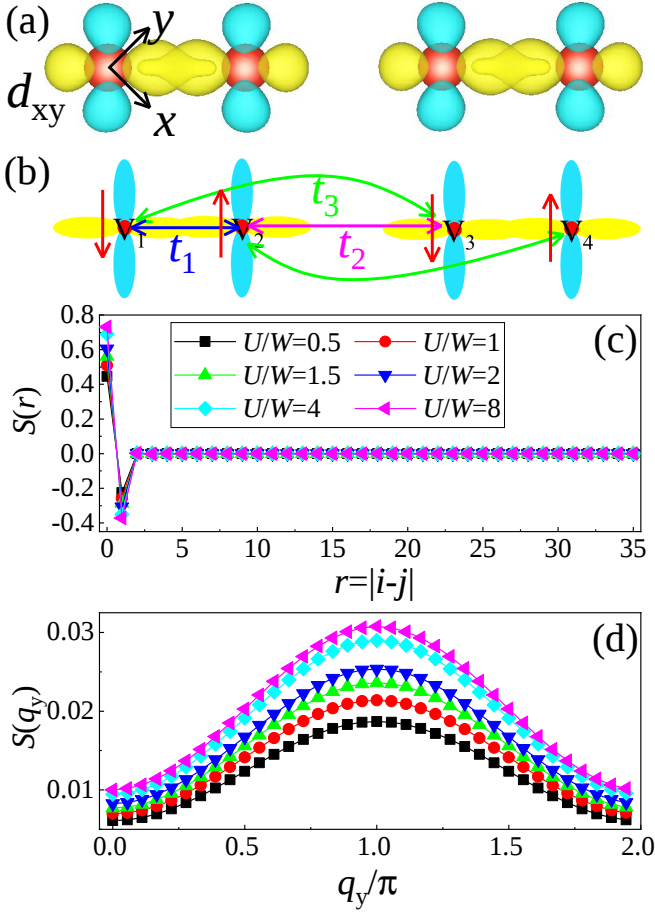
FIG. 5. (a) Wannier function of the V 3d_{xy} orbital, indicating the alternating d\sigma -bonding and d\sigma^* -antibonding states along the b -axis. (b) Different hoppings along the chain used in our DMRG calculations ( t_1 = -0.647 eV, t_2 = 0.067 eV and t_3 = 0.009 eV). All the hopping amplitudes were obtained from the DFT calculations via Wannier functions. The spin arrows represent short-range antiferromagnetic-antiferromagnetic coupling along the chain. (c) S(r)=\langle \mathbf{S}_i \cdot \mathbf{S}_j \rangle (with r=|i-j| ) and (d) S(q_y) for different values of U/W . Here, we used a 36-sites cluster chain with two nearest-neighbors and one next-nearest-neighbor hoppings. (d) Spin structure factor at the six values of U/W of panel (c).
