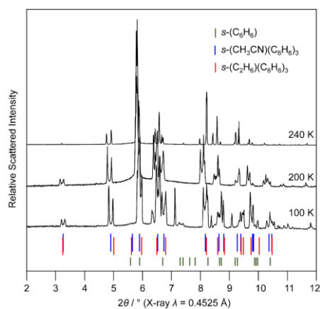
Fig. 3 Powder diffraction patterns of a system made of acetonitrile and benzene in a 1:3 ratio, crystallized in an environment saturated with liquid ethane.
