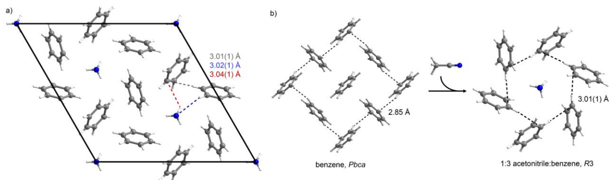
Fig. 2 a) Crystal packing diagram of the 1:3 acetonitrile:benzene cocrystal. b) Fragments of the crystal packing diagrams of benzene and the cocrystal schematically representing the peritectic phase transition. Legend: nitrogen in blue, carbon in grey, hydrogen in white.
