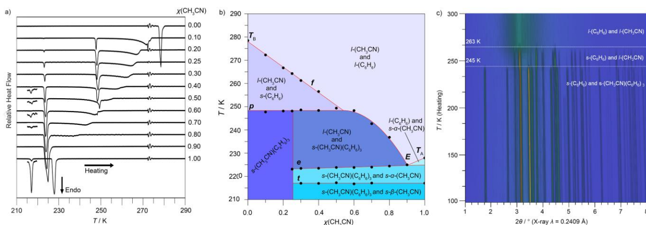
Fig. 1 a) DSC curves of mixtures of benzene and acetonitrile and their b) \chi - T phase diagram. The composition of the condensed phase regions was determined from the c) X-ray diffraction data collected upon heating of 1:3 sample of acetonitrile and benzene.
