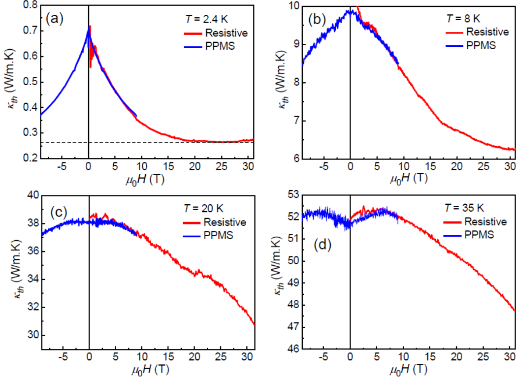
Figure 2: (Color online) Thermal conductivity \kappa_{th} of YIG as a function of the magnetic field measured at several temperatures both in a PPMS and in a resistive magnet.
