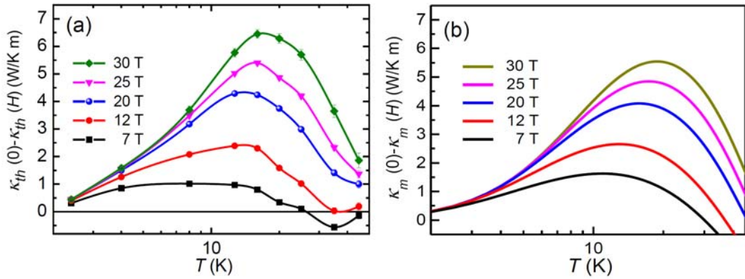
Figure 4: (Color online) (a) Difference between the thermal conductivities measured at zero field and under selected field values as a function of the temperature. (b) Temperature dependence of the calculated magnon thermal conductivity in YIG as function of the temperature and for several field values.
