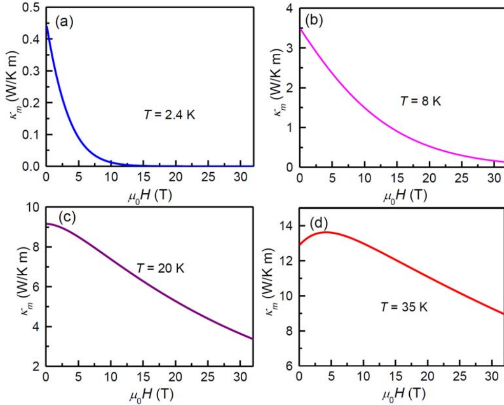
Figure 3: (Color online) Thermal conductivity in YIG as a function of the magnetic field at several temperatures and as calculated from Eqs. (1)-(3).
