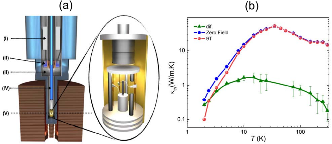
Figure 1: (a) Schematic illustration of the apparatus and sample holder used for measuring the thermal conductivity \kappa_{th} of YIG at high magnetic fields, showing: (I) Sorb used both for injecting the exchange-gas and for producing high vacuum in the sample space; (II) 1K pot used to condense ^3\text{He} inside the cold finger; (III) Sample space; (IV) Cold finger; and (V) Center of the magnet with the sample holder. The zoom in shows the sample holder with the YIG sample, the silver wires attached to the heater, and the Cernox thermometers, identified by the letters: T - thermometers, L - thermal link, H – heater, and S - sample. (b) Temperature ( T ) dependence of \kappa_{th} measured in the PPMS under zero field (blue pentagons) and under a magnetic field of 9 T (red circles). The corresponding reduction in \kappa_{th} with the field is represented by the green triangles.
