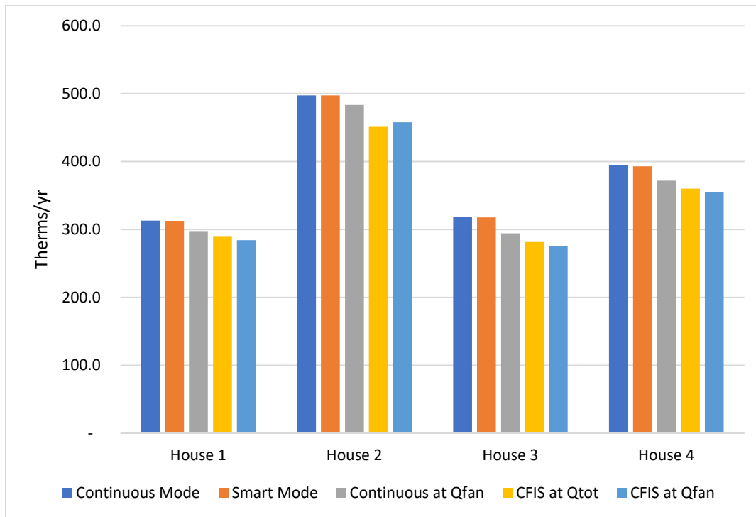
Figure 39. Uncorrected BEopt model annual therm usage results for the five ventilation options
