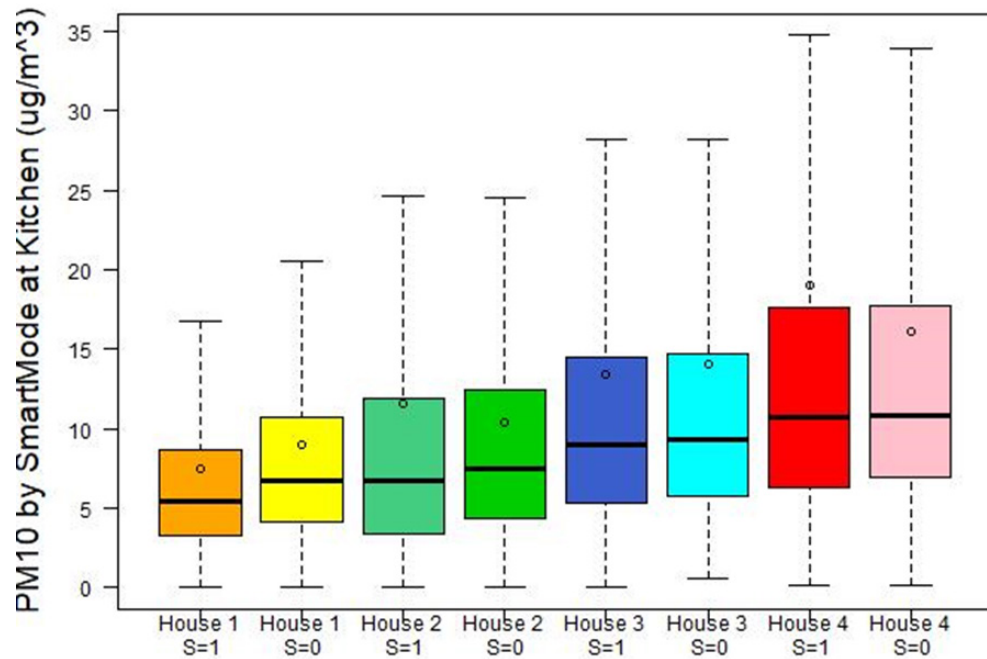
Figure 34. \text{PM}_{10} results in the kitchen by ERV mode (S = 1 refers to ERV Smart Mode; S = 0 refers to ERV Continuous Mode)
