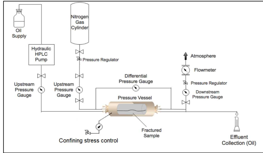
Figure 1. Schematic of the flow test configuration
