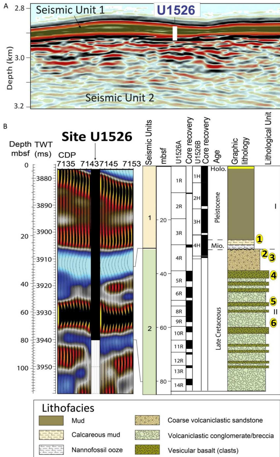
Fig. S4. Enlarged seismic section of the crest of Tūranganui Knoll seamount, in the vicinity of IODP Site U1526, and lithological log tied to the seismic data. (A) The seismic data are located on Fig. 2B. (B) Composite log derived from coring at Holes U1526A and U1526B. Bold numbers with yellow background show the location of photographs in Fig. 4B.
