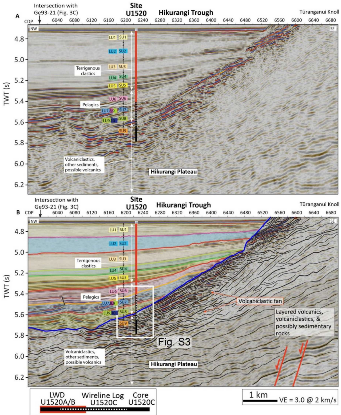
Fig. S2. Seismic reflection profile across the eastern side of the Hikurangi Trough and buried lower flank of Tūranganui Knoll seamant in the vicinity of IODP Site U1520. (A) Un-interpreted section. (B) Interpreted section. Black line work highlights reflection architecture within the subducting Hikurangi Plateau. LWD, logging-while-drilling. SU, seismic unit. LU, logging unit. White box indicates the region addressed in Figure S3.
