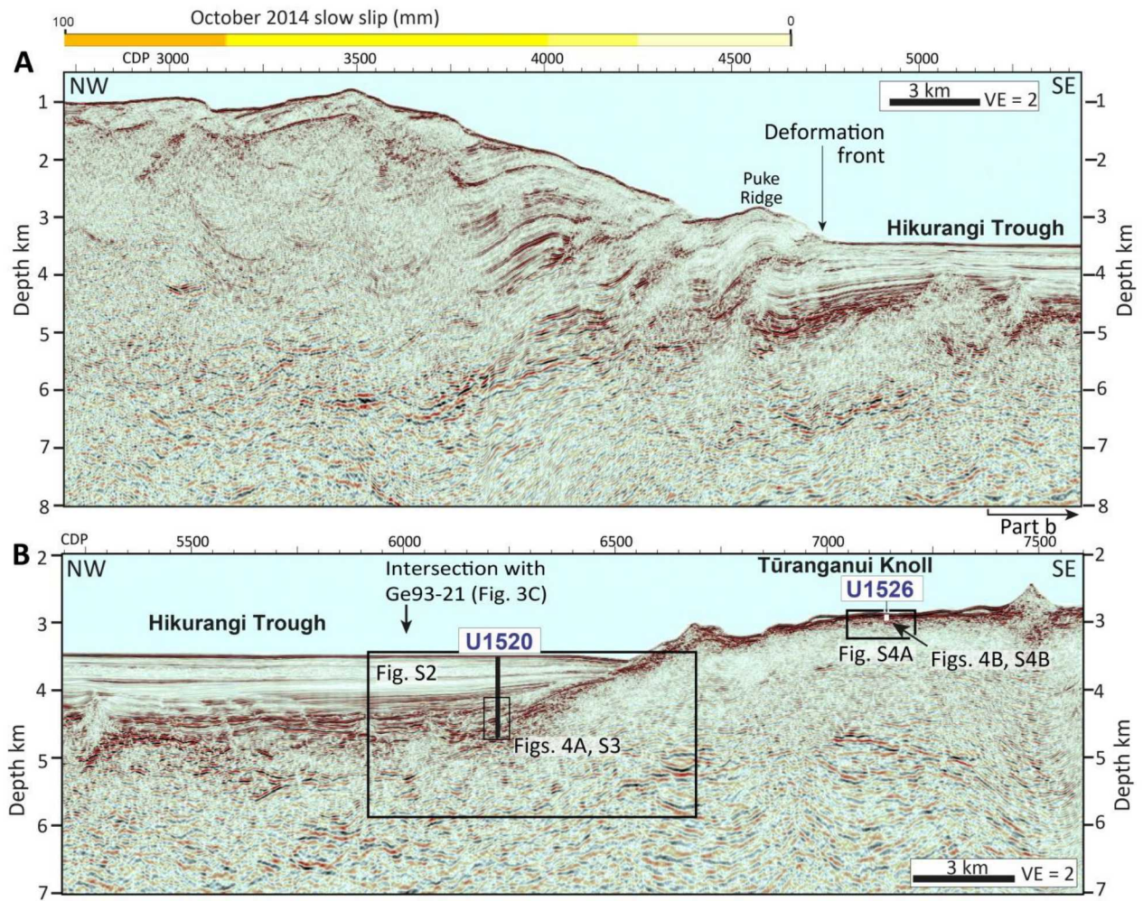
Fig. S1. Uninterpreted panels of seismic line 05CM-04. See Fig. 2 for interpretation.
