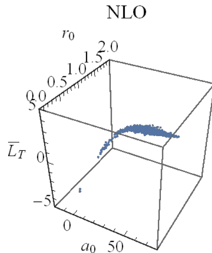
FIG. 6: a_0 - r_0 - \bar{L}_T 3-dim scatter plot based on MCMC sampling. All three axes have units of fm.
