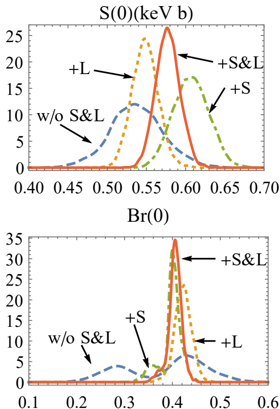
FIG. 4: The impact on S(0) and Br(0) of analyzing subsets of our full data set. The blue-dashed “w/o S & L” curve is the result if Seattle and Luna data are both excluded, while the orange-dashed “+ L” and green-dot-dashed “+ S” curves show the result when that analysis is supplemented with the Luna and Seattle data respectively. The solid curve “+S & L” curve is our final NLO result, including all data sets described above.
