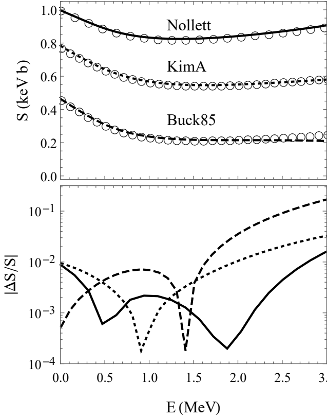
FIG. 1: Total S factors in different potential models and EFT fits thereto. The full S factor produced by each model is represented by the open circles in the upper panel. The models are Nollett [13], KimA [36] and Buck85 [34]. For readability, the first two results are shifted vertically by 0.6 and 0.3 keV b respectively. The solid, short-dashed, and long-dashed lines represent the partial-N4LO EFT fits to the model results, i.e., the fits whose optimal parameter values are listed in Table I. The lower panel shows, on a log-linear scale, the fractional discrepancy vs energy, \Delta S(E)/S(E) , between each full model result and the corresponding EFT fit: Nollett (solid), KimA (short dashed), and Buck85 (long dashed).
