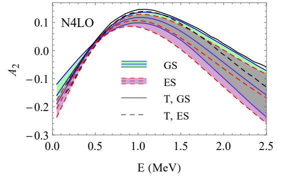
FIG. 11: Solid blue (dashed red) lines indicate the mean and 68% interval for the anisotropy factor for the capture to the GS (ES) in the partial-N4LO MCMC samples. Green (purple) fills in the 68% region. The black solid (GS) and dashed (ES) are the anisotropy calculation of Ref. [49].
