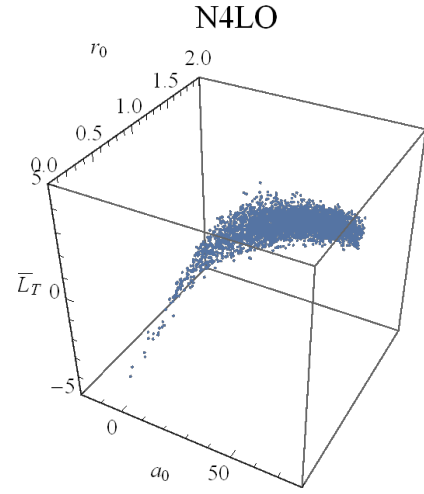
FIG. 10: a_0 - r_0 - \bar{L}_T (all in units of fm) three-dimensional scatter plot based on the partial-N4LO MCMC ensemble.
