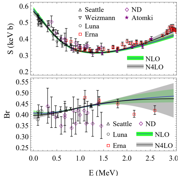
FIG. 2: Total S -factor and branching-ratio results. The data sets are denoted as in the legend and are from Luna [57–60], Erna [61], Seattle [55], Weizman [56], Atomki [16], and Notre Dame (ND) [15]. The green (gray) band shows the 68% interval for S(E) and Br(E) in our NLO (partial-N4LO) analysis. The mean is denoted by the blue (black) line.
