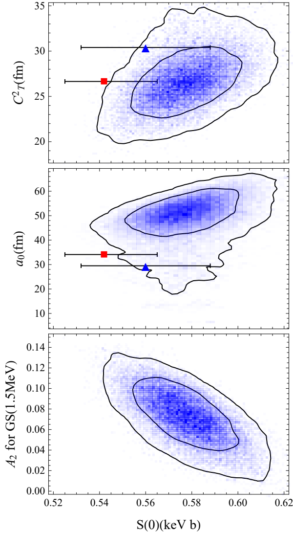
FIG. 7: NLO correlation of S(0) with C_T^2 , a_0 , and A_2 of the ground-state transition at 1.5 MeV. In the top panel, the red square and blue triangle denote C_T^2 and S(0) from Refs. [17] and [11] (only uncertainty for S(0) quoted). The values of a_0 and S(0) from Refs. [11, 17] are also shown in the middle panel (again, only uncertainty for S(0) is shown).
