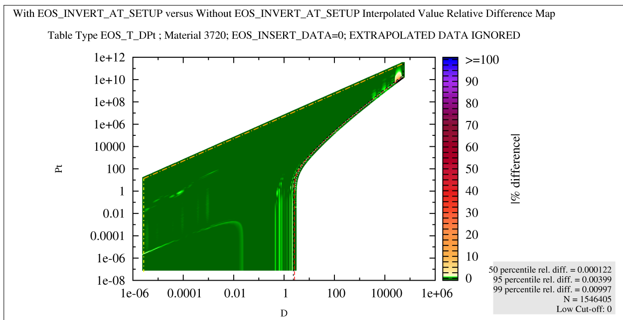
Figure 9.10: Color map of relative differences comparing the interpolation of T(\rho, P_t) , which was calculated using both of EOSPAC 6's default and pre-inverted (i.e., EOS_INVERT_AT_SETUP) inverse interpolation modes.
