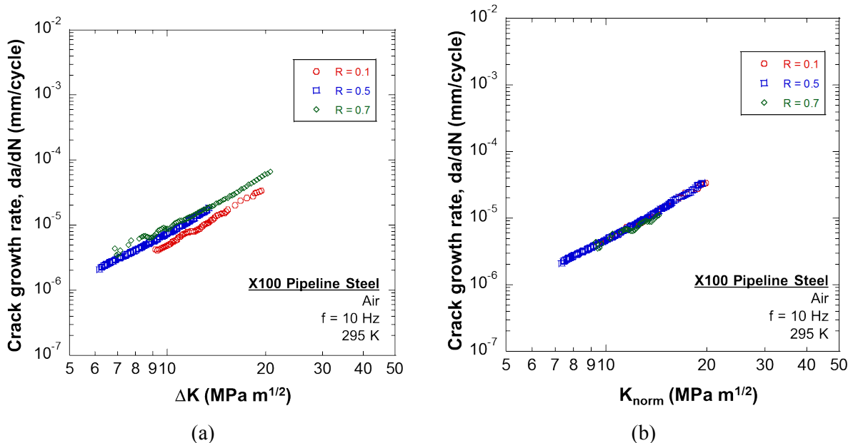
Figure 4 – (a) FCGR curves for X100 base metal performed in air at 10 Hz, (b) Fatigue crack growth rate data versus K_{norm} for data from (a) according to Eq. 3 using n = 0.25 .
