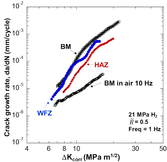
Figure 11 – Residual stress-free FCGR curves ( da/dN versus \Delta K_{corr} ) for X100 base metal (BM), weld fusion zone (WFZ), and heat affected zone (HAZ).
