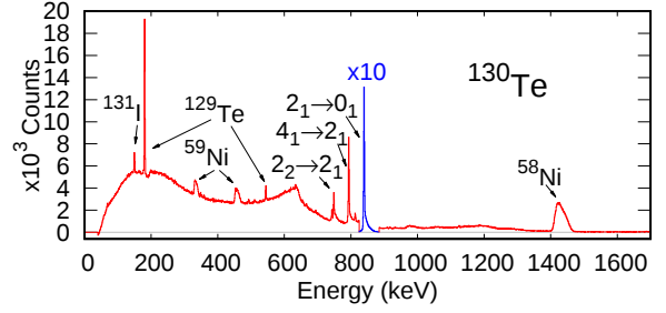
Figure 1. Energy spectrum taken at 65^\circ in Run F as defined in Table 1 (enriched ^{130}\text{Te} target). The decay of the first excited state has been scaled down by a factor of 10.
