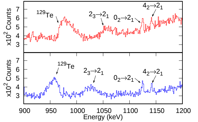
Figure 2. Spectra for the region from 900 to 1200 keV in Run F as defined in Table 1 (enriched ^{130}\text{Te} target). The top and bottom panels display data from 65^\circ and 115^\circ detectors, respectively.
