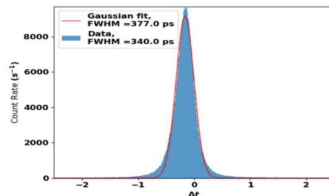
Fig. 5. Na-22 time difference histogram (units of ns).
