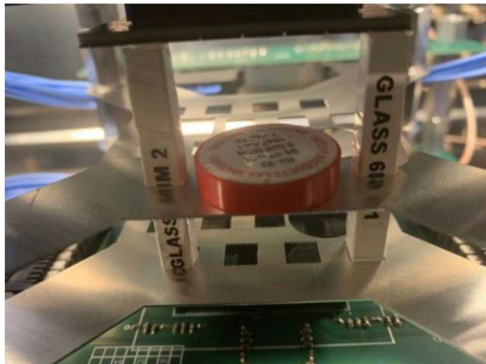
Fig. 3. Na-22 time resolution measurement with two organic glass bars.
