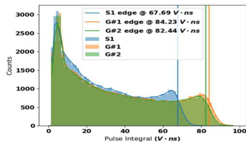
Fig. 4. Cs-137 spectra for stilbene and glass cubes.
