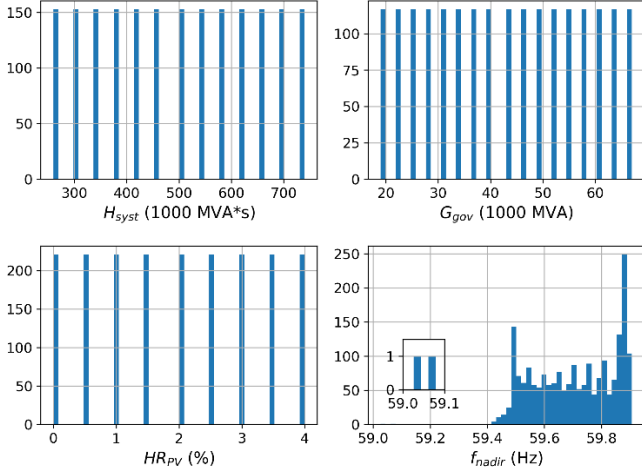
Fig. 6. Histograms of features.
