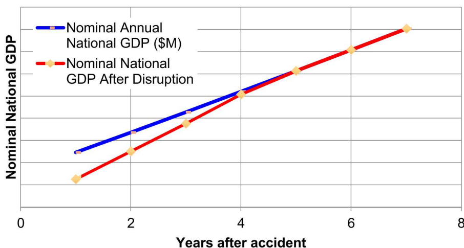
Figure 3. Nominal GDP recovery at the national scale assuming the GDP growth rate is higher than the social discount rate. Here the national GDP fully recovers to its pre-accident trajectory at the beginning of the 5 th year after the accident.
