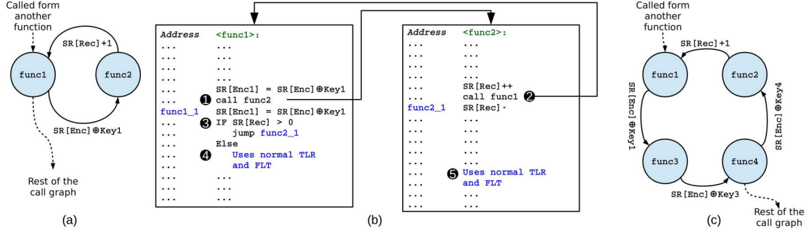
Fig. 14. Illustration of handling indirect recursion. Fig.(a) shows a call graph of two indirect functions. Fig(b) shows a pseudo code of instrumenting indirect functions. Fig(c) illustrates a cycle of four functions. Functions func1 and func2 are handled in the same method as the first case in(a).
