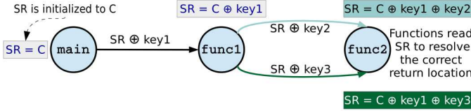
Fig. 1. Illustration of encoding SR through an XOR chain. Arrows indicate a call site in the call graph. SR is XORed each time an edge is walked.
