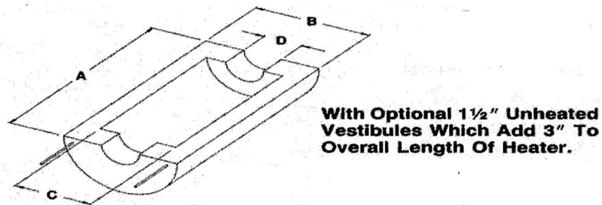
Figure 1: Ceramic Fiber Heater
