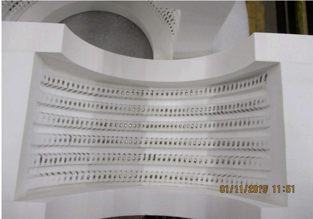
Figure 2: Ceramic Fiber Heater
