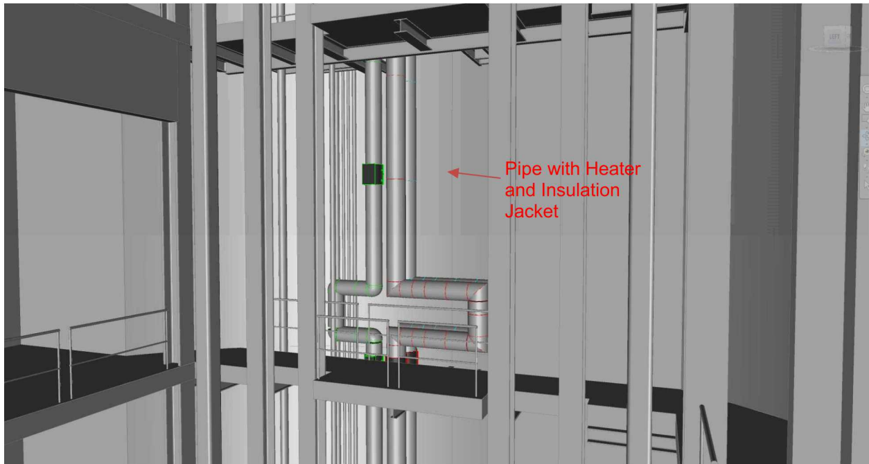
Level 180 Insulated Piping with CF Heater: Ullage Gas Equalizer, Molten Salt Hot and Cold Piping Expansion Loop.
