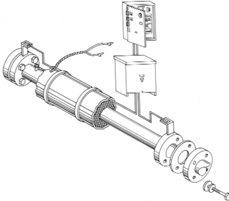
Figure 8: Impedance Heating System
