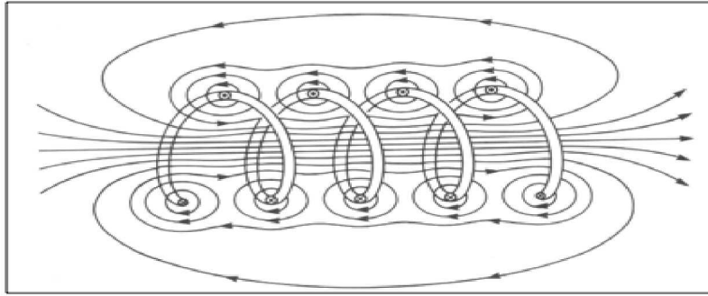
Figure 9: Inductance Heating System
