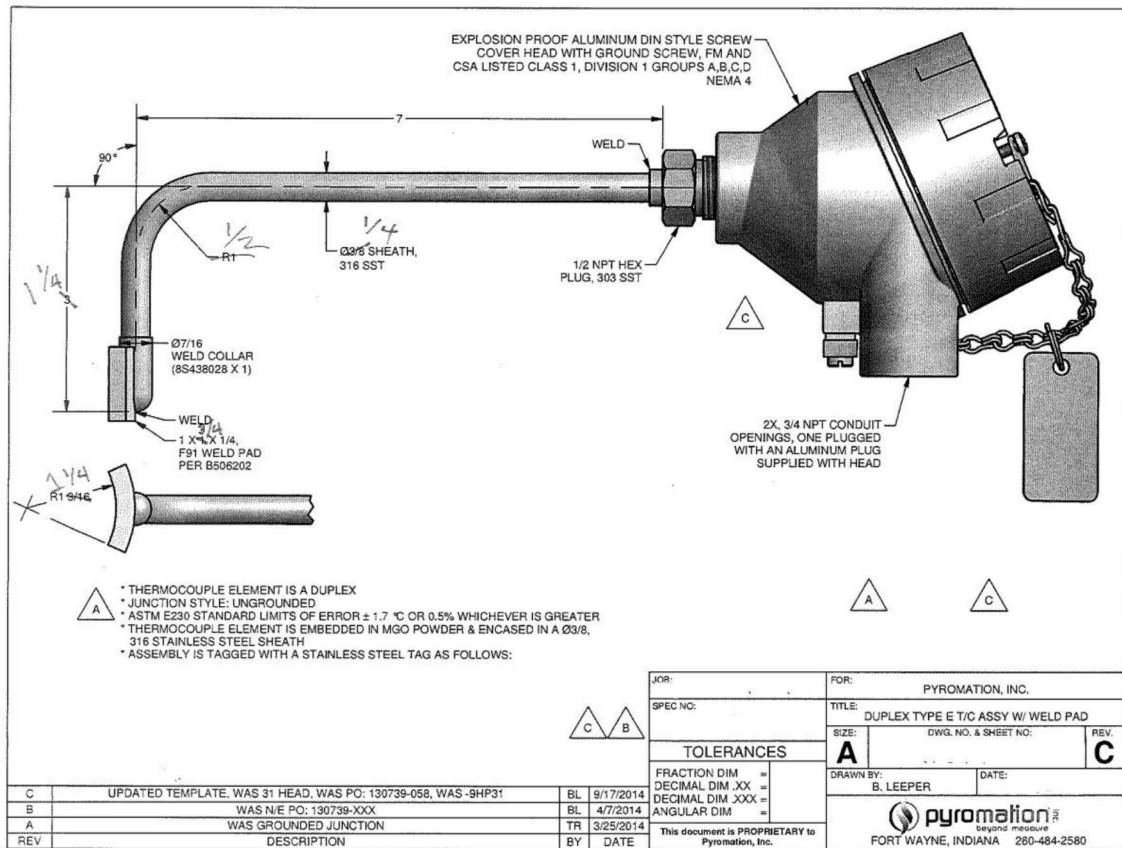
Figure 3: Pyromation Type E Thermal Couple
