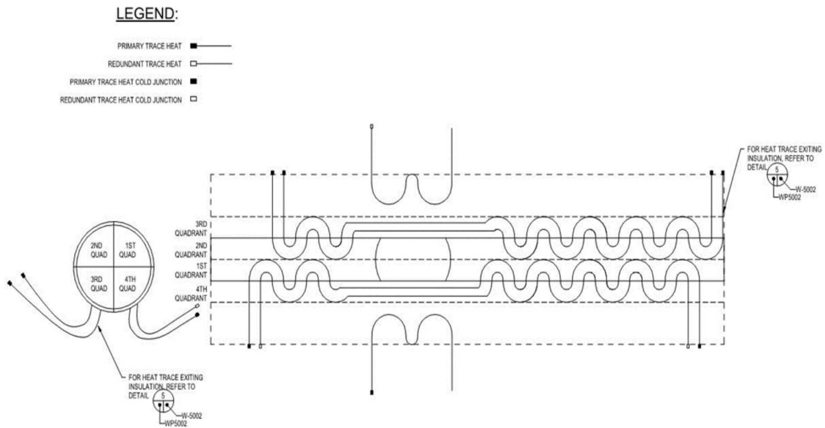
Figure 5: MI Cable Serpentine Pattern Detail
