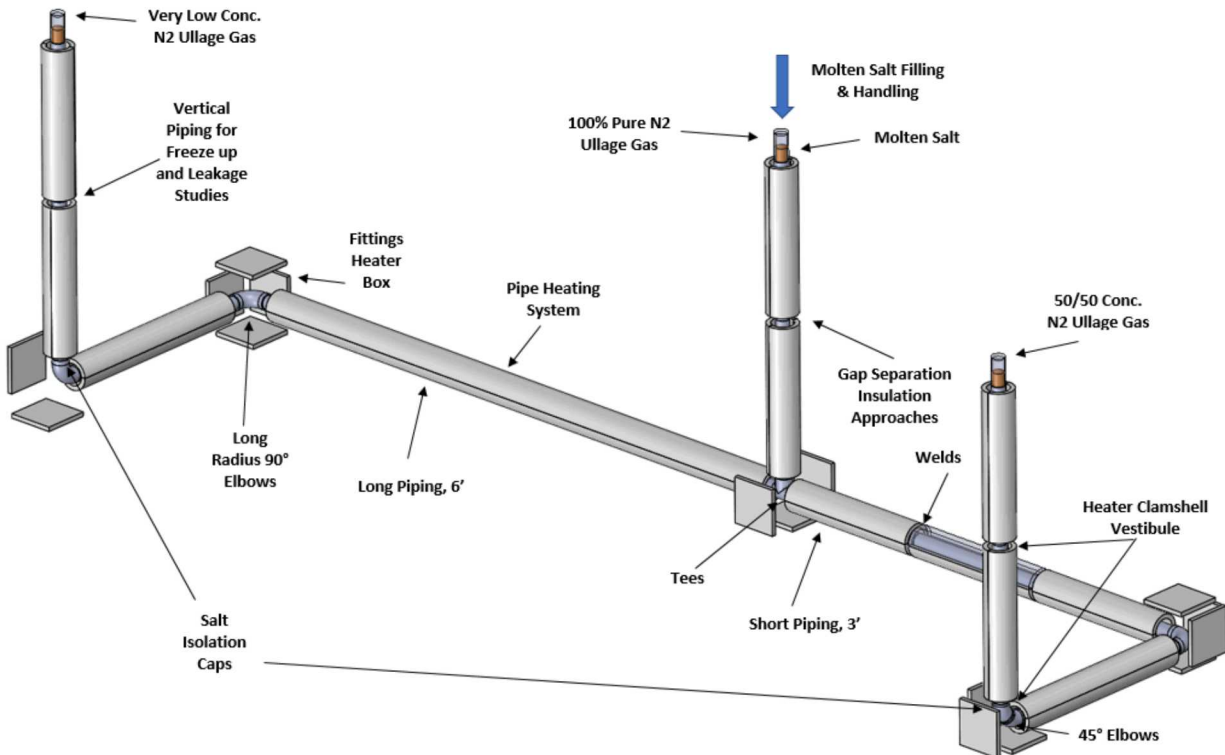
Figure 10: Phase 1B Test Setup for Thermal Transport Pipe Heating Investigations.
