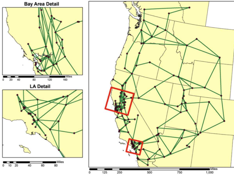
Fig. 1 Illustration of the WECC 240-bus system [42].
