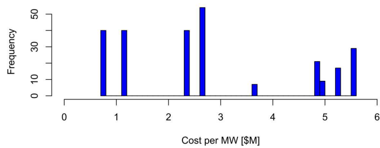
Fig. 3 Histogram of generation capital costs per MW.
