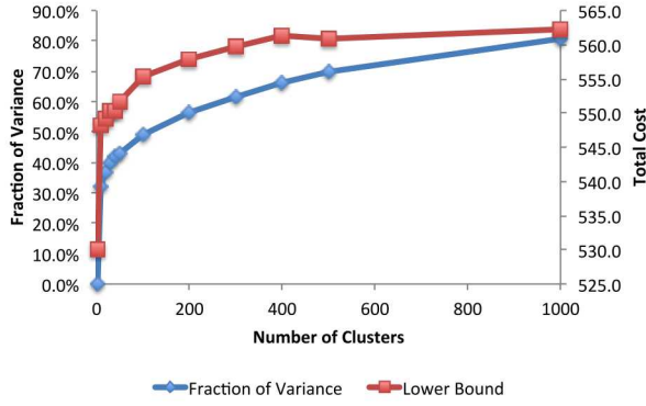
Fig. 2 Fraction of variance captured relative to the full dataset and objective function value of the LP relaxation of the investment-planning problem as a function of the number of clusters.
