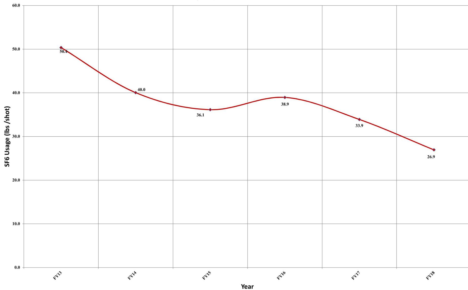
Z Machine SF 6 Usage in Annual Pounds Per Shot
