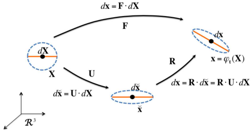
Figure 5-2. Physical interpretation of the polar decomposition. (Dotted outline indicates infinitesimal neighborhood of point X .)
