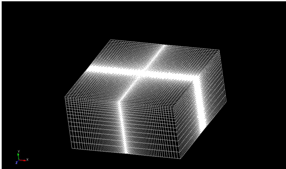
Figure 1-19. Graded Mesh
