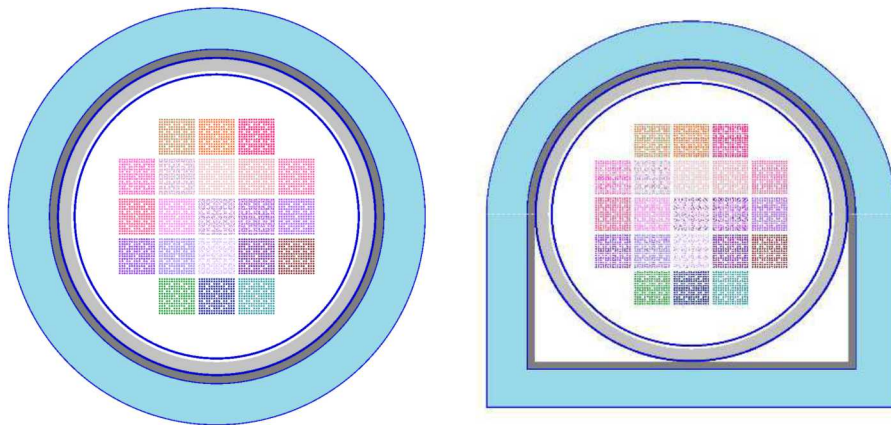
Figure 6-8. Alternative supplemental shield geometries.
