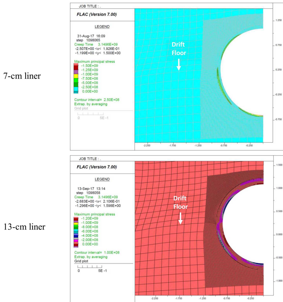
Figure B-3. Maximum principal stress for the liner thicknesses indicated, and packages emplaced into semi-cylindrical cavities in the tunnel floor.
