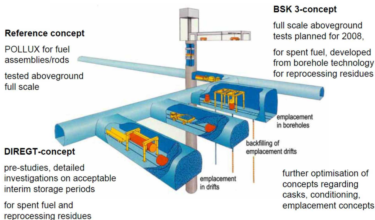
Figure 2-1. Gorleben disposal concepts for consolidated SNF rods in POLLUX casks (reference concept) and BSK casks (emplacement in boreholes), and for intact fuel in CASTOR casks (DIREGT concept) (from Bollingerfehr and Filbert 2010).
