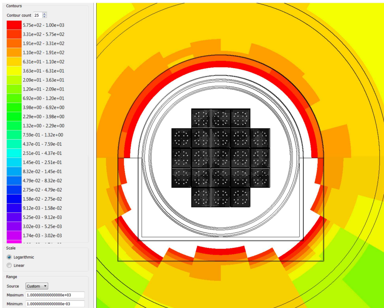
Figure A-7. Total dose rate map (mrem/hour) for cask with 19-MT gamma shield, and 21-MT neutron shield.
