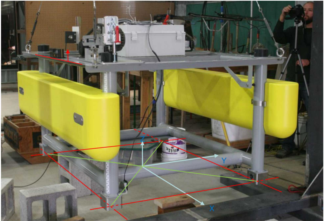
Figure 5-9. Reference Photo for Platform COG Calculation
