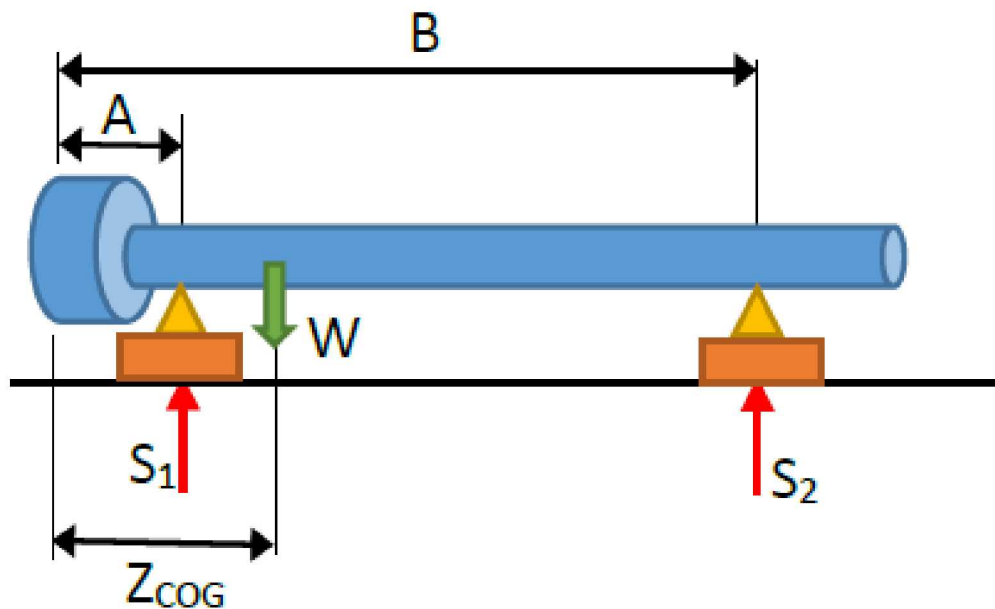
Figure A-1. Center of Gravity Measurement Setup Scale
