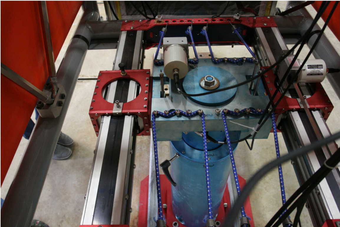
Figure 6-2. Platform Stabilizing Supports (diagonal bars on left side)
