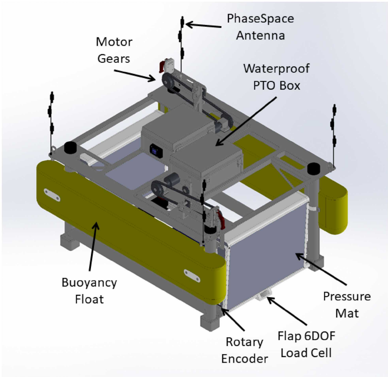
Figure 5-1. FOSWEC Mechanical Design Rendering (Phase 1)
