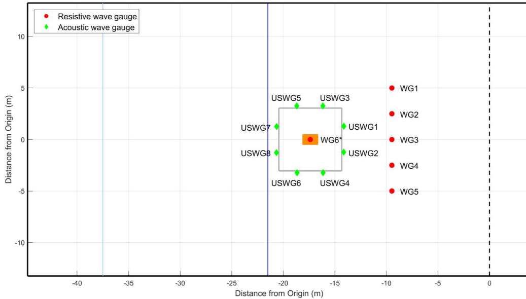
Figure 3-8. The layout of the DWB during testing, showing the location of the wave gauges, test frame (gray) and the FOSWEC device (orange rectangle). Note that wave gauge 6 (WG6) was only in place for wave calibration tests, when the FOSWEC device was not in the basin. The origin is the middle of the wave maker, indicated by the dashed line. The initiation of the beach (dark blue) and the SWL (light blue) are also indicated.
