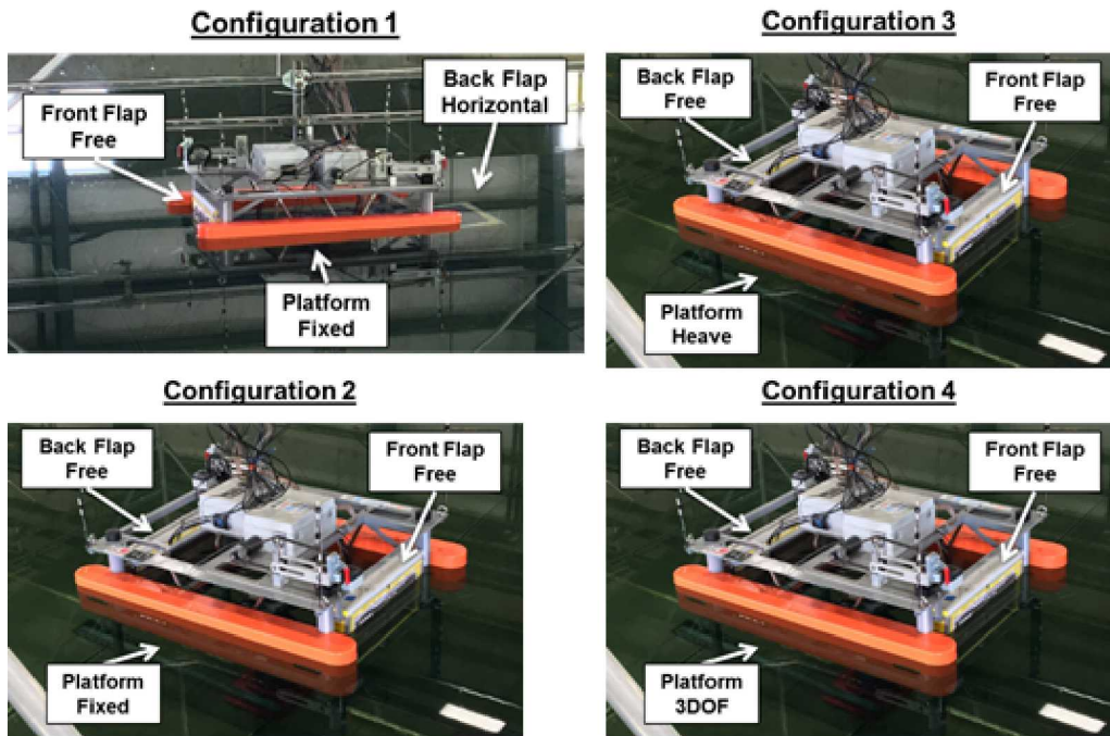
Figure 3-6. FOSWEC configurations (Config 1 - Config 4)
