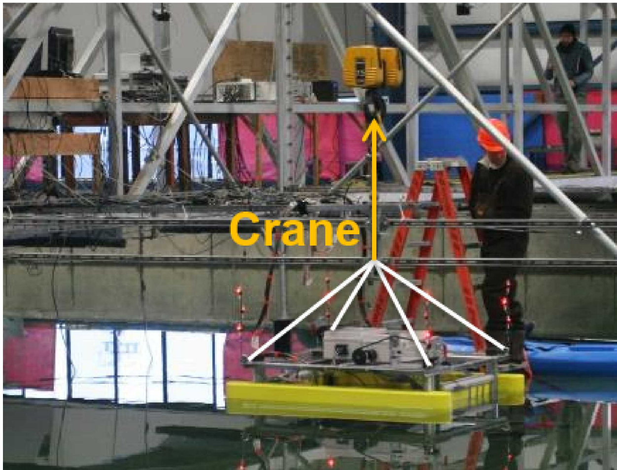
Figure 5-10. Heave Decay and Static Offset Setup
