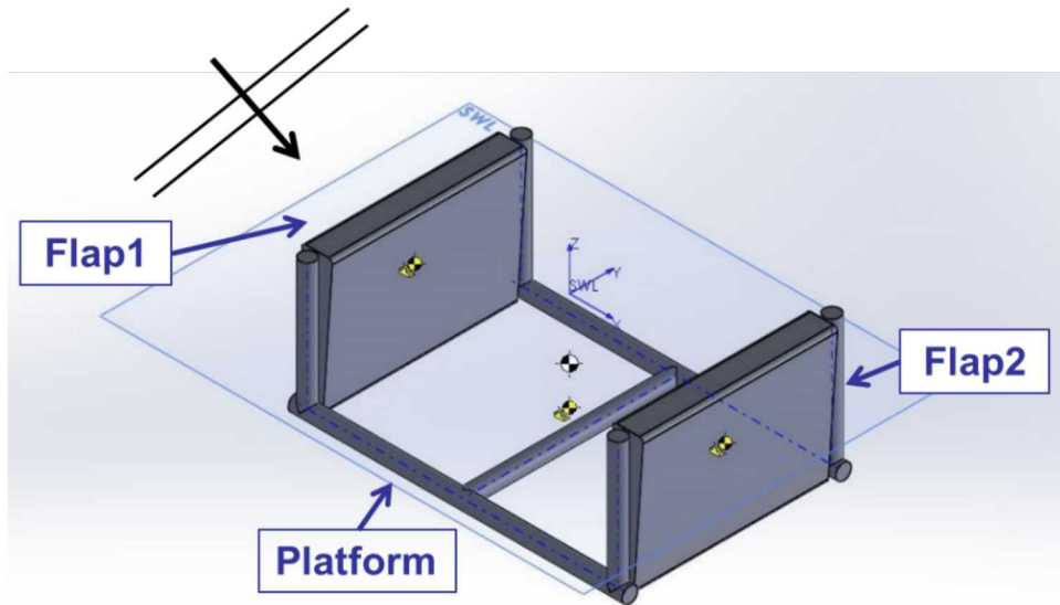
Figure 3-4. FOSWEC hydrodynamic design concept
