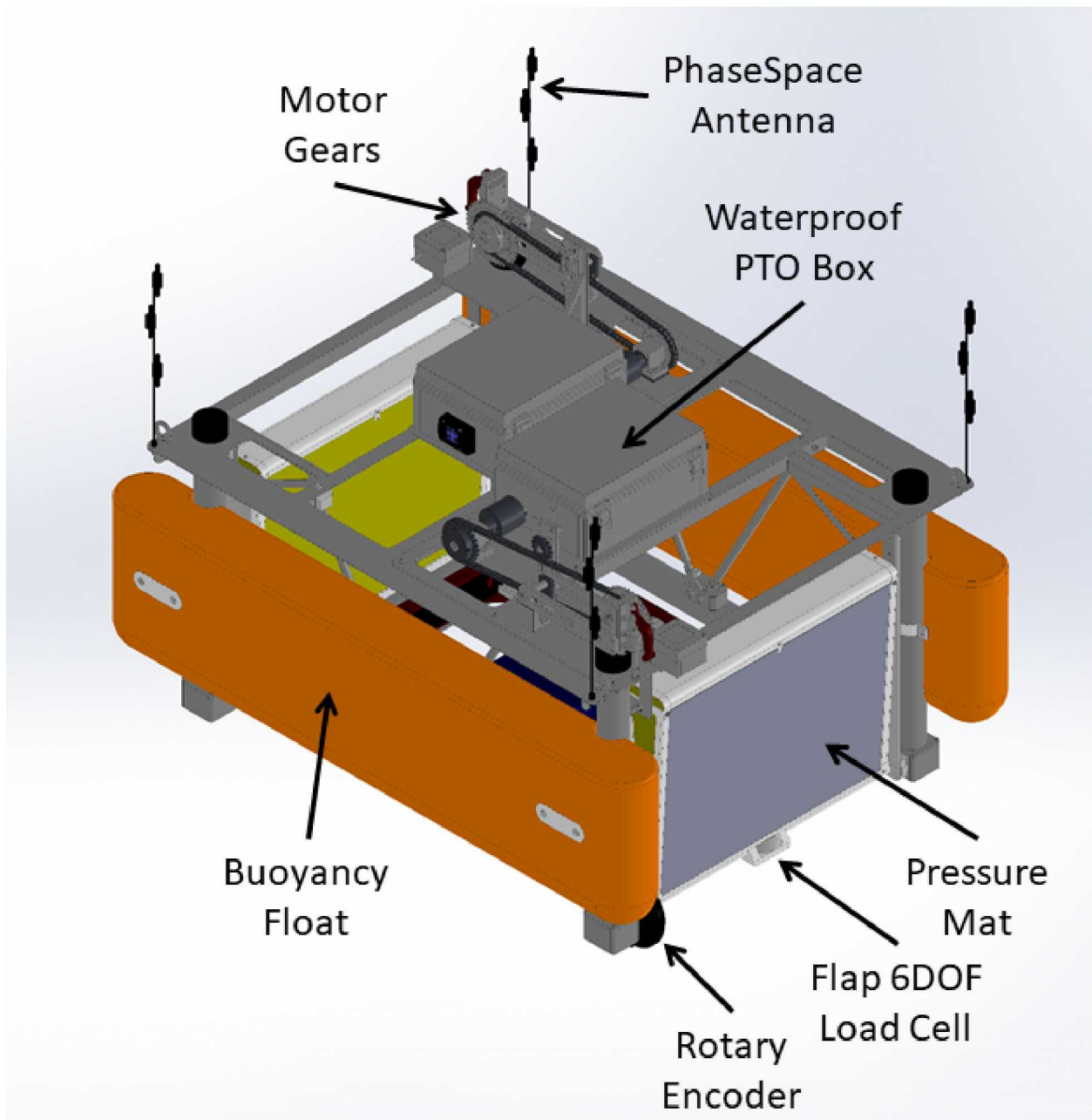
Figure 7-1. FOSWEC Mechanical Design Rendering (Phase 2)
