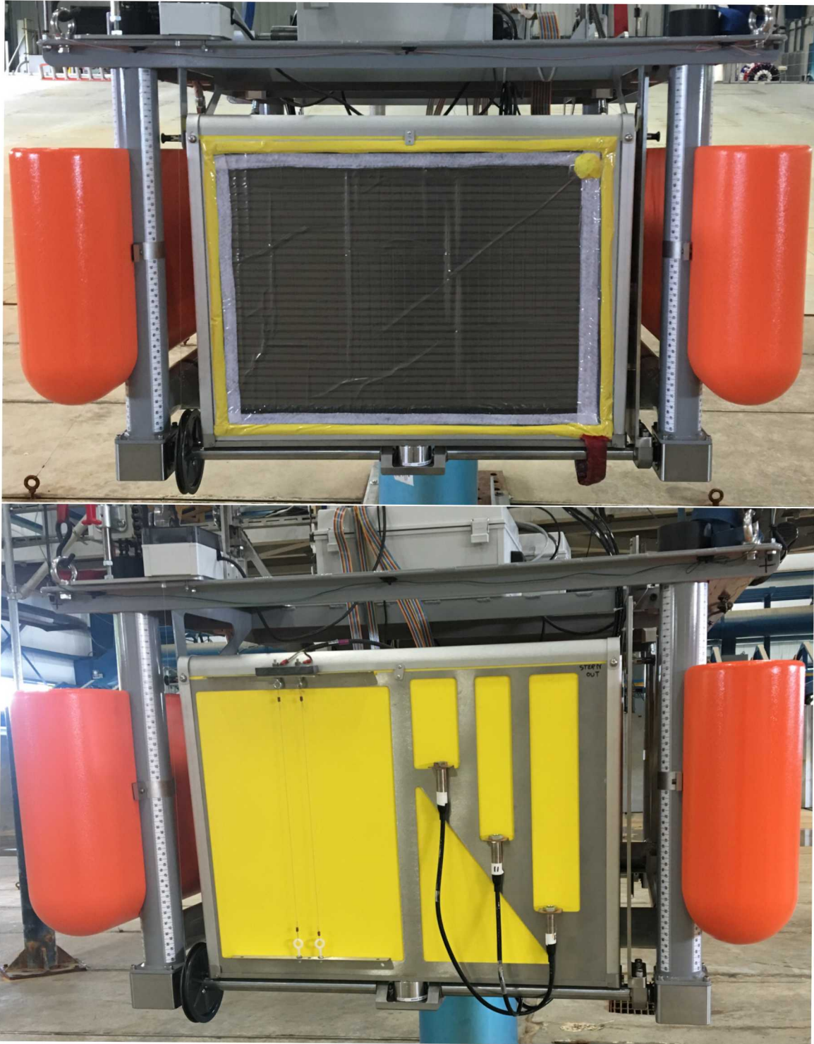
Figure 6-3. Flap Locking Mechanism (vertical bar on right side of flap) and Pressure Mat Waterproofing (top image)
