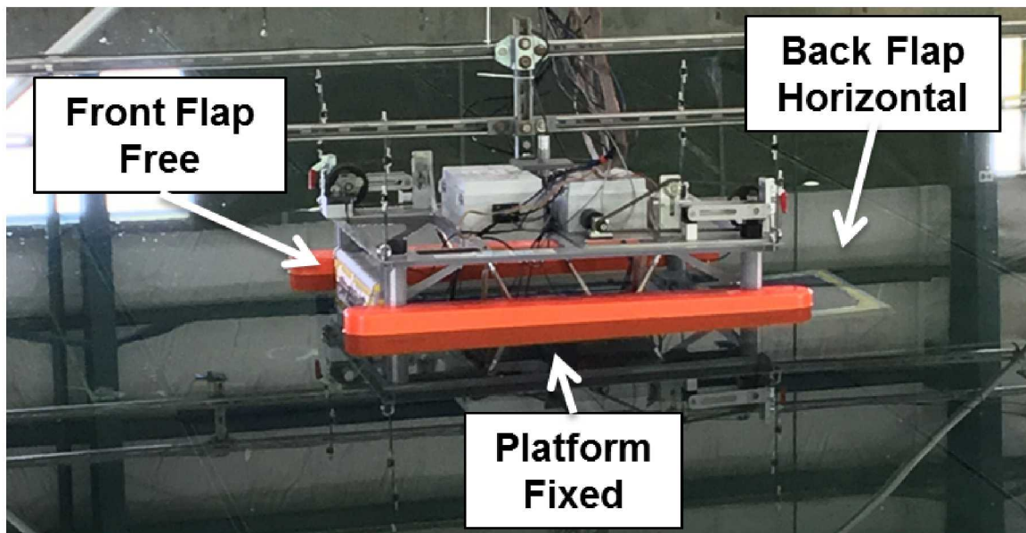
Figure 7-5. FOSWEC Config 1 (Phase 2)
