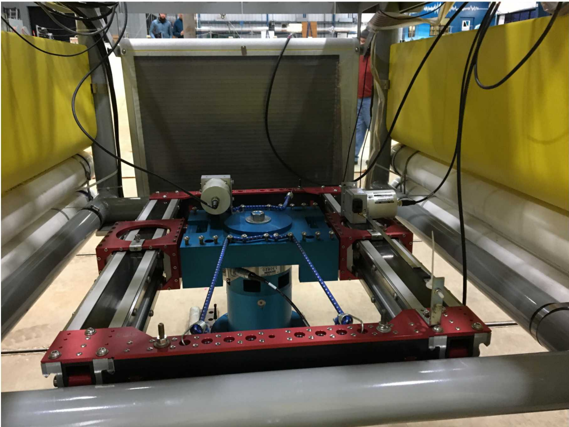
Figure 5-7. Interior view of Arm/FOSWEC Assembly
