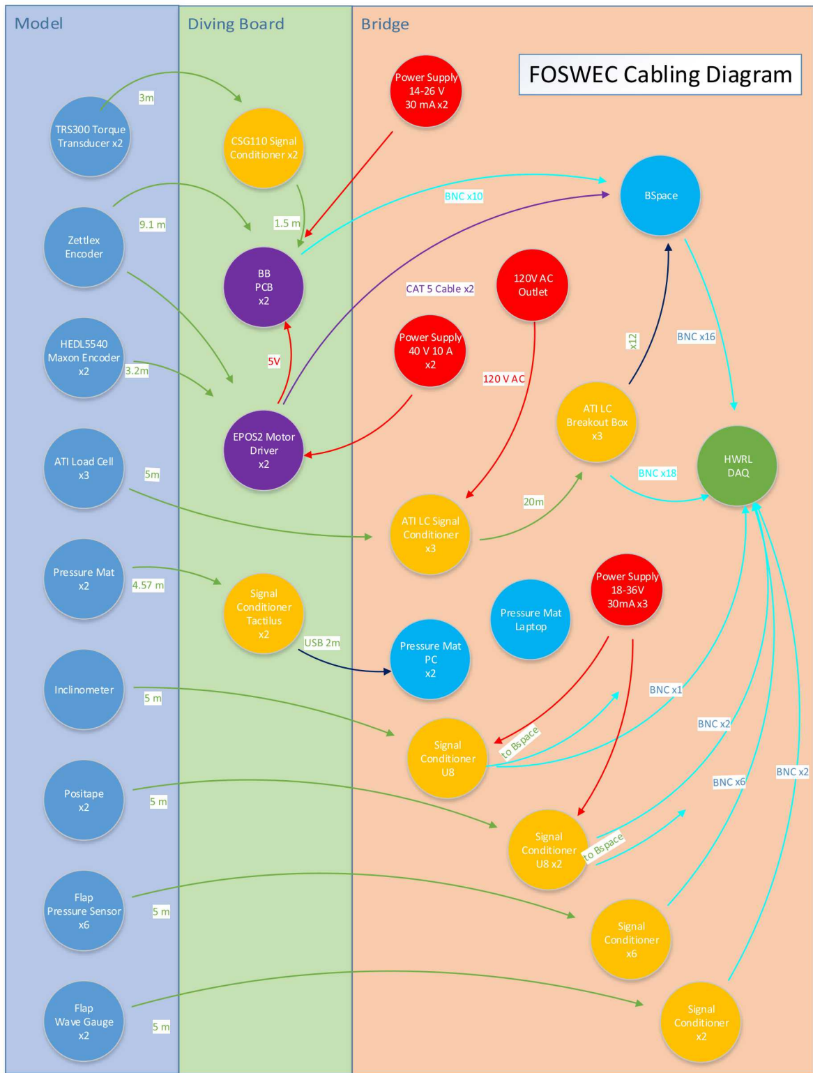
Figure C-2. FOSWEC Cabling Diagram (Phase 2)
