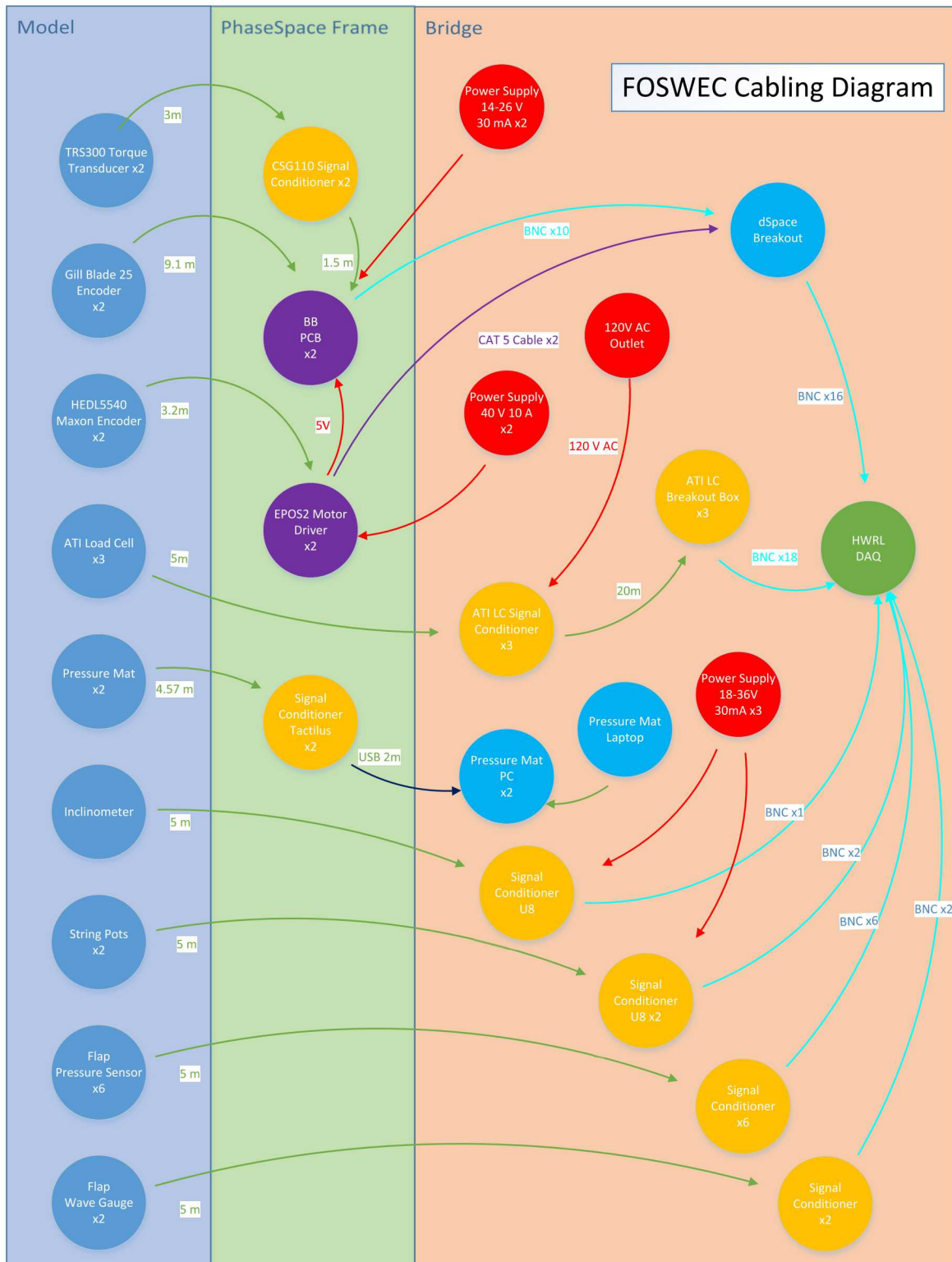
Figure C-1. FOSWEC Cabling Diagram (Phase 1)
