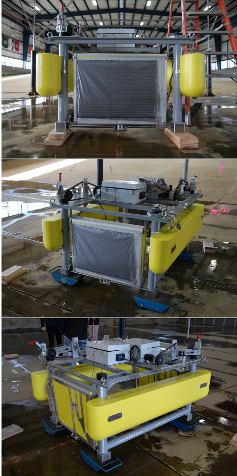
Figure 5-3. FOSWEC before installation (Phase 1)
