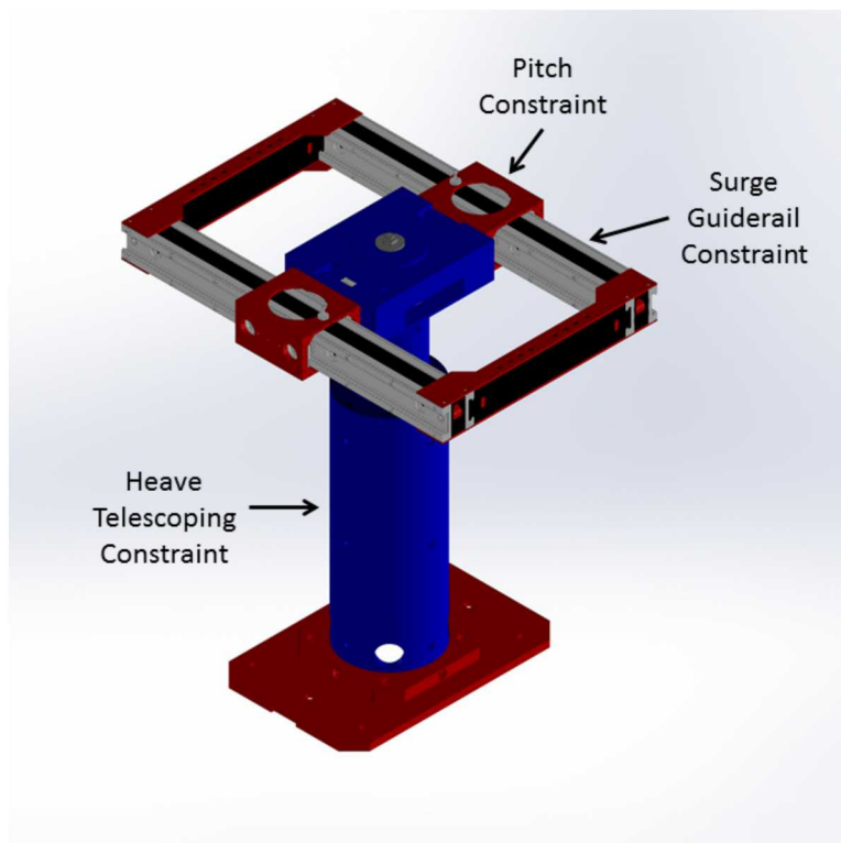
Figure 5-4. Arm Rendering (Phase 1)
