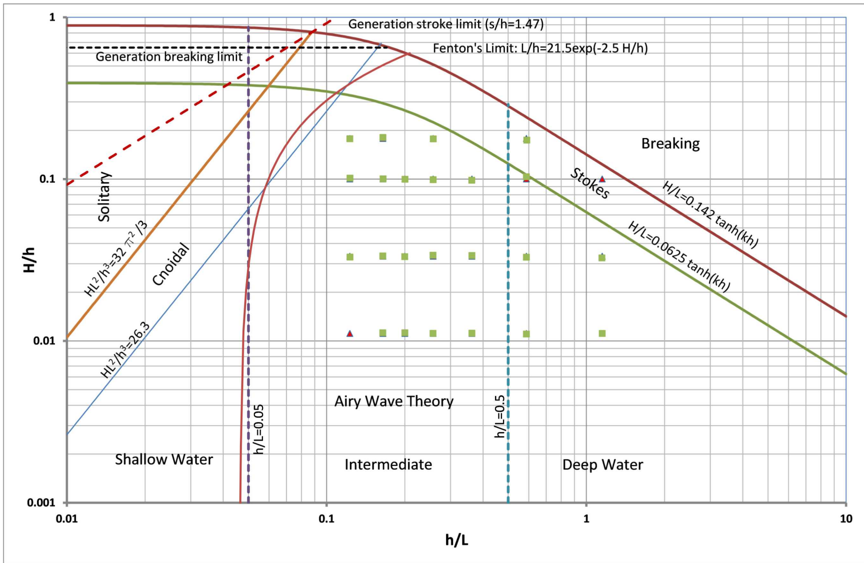
Figure 4-1. Regular Wave Calibration Results (red triangles are targeted, and green squares are observed)
