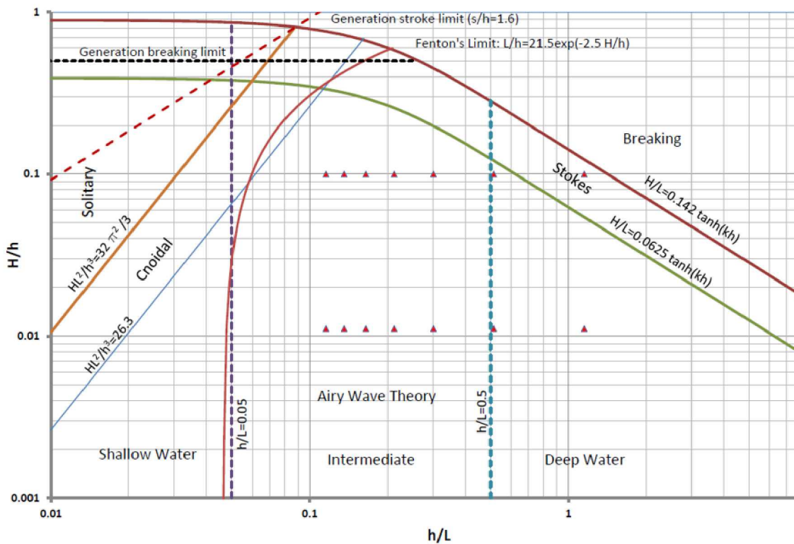
Figure 2-1. HWRL DWB 1:33 Scaling Analysis
