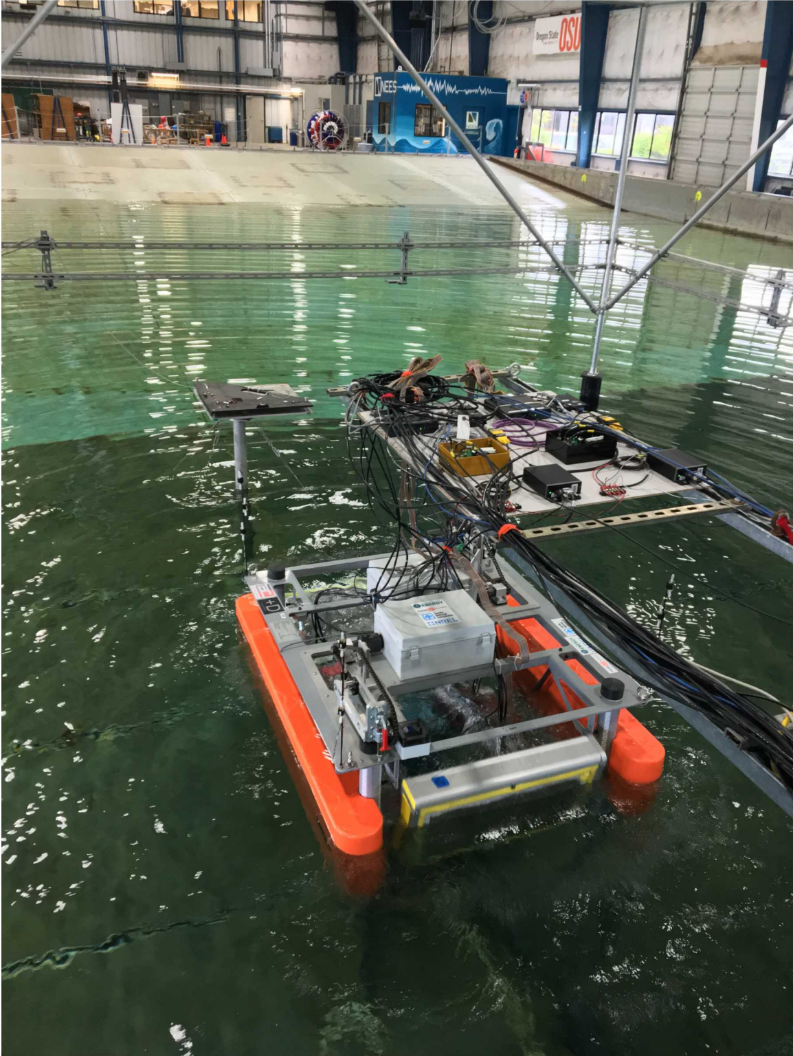
Figure 7-4. Forced Oscillation Experiment (Phase 2)
