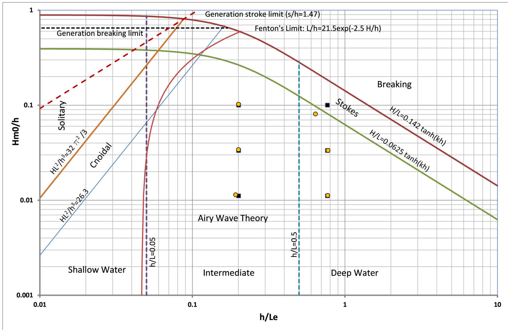
Figure 4-2. Irregular Wave Calibration Results, Averaged (orange circles are targeted, and black squares are average observed)
