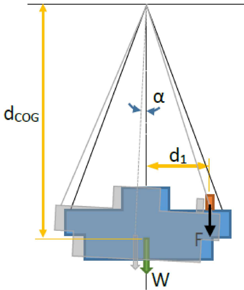
Figure A-2. Pendulum Method for COG
