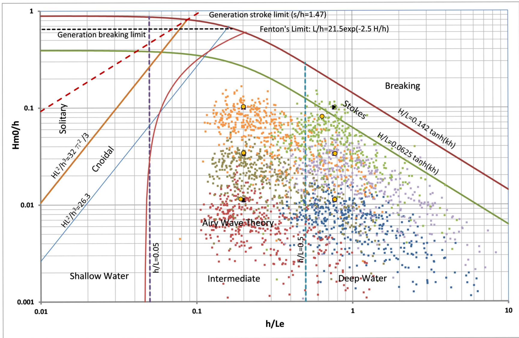
Figure 4-3. Irregular Wave Calibration Results, Detailed (orange circles are targeted, black squares are average observed, colored dots are the individual wavetrains for each sea state)
