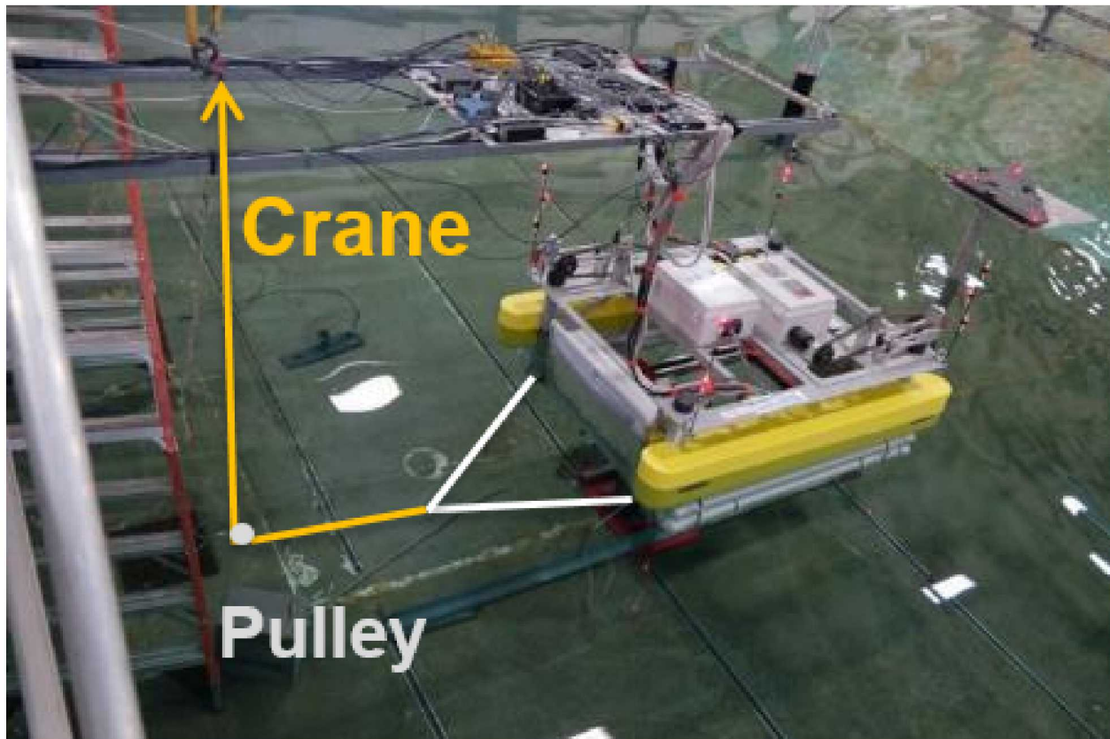
Figure 5-12. Surge Decay and Static Offset Setup
