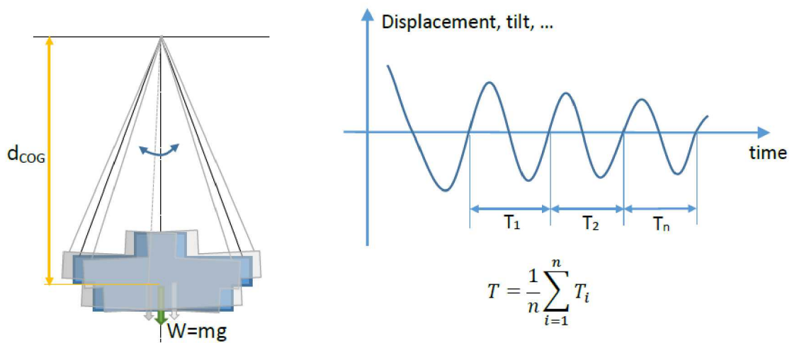
Figure A-3. Reference for MOI Calculation
