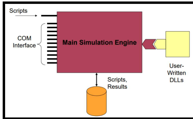
Figure 9: Structure of OpenDSS platform [19].
