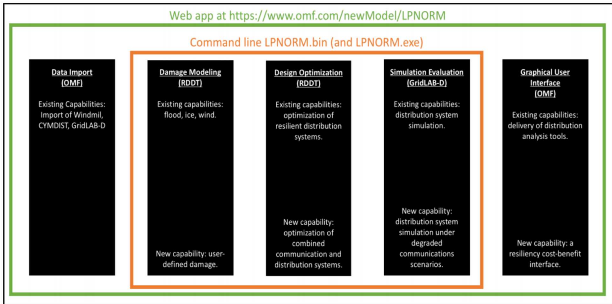
Figure 7: LPNORM system architecture [10].
