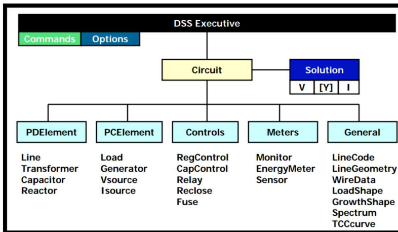
Figure 10: Object structure of OpenDSS platform [19].
