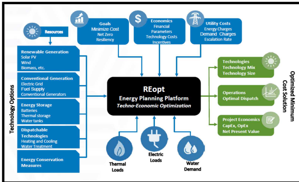
Figure 6: Visualization of REopt framework [9].
