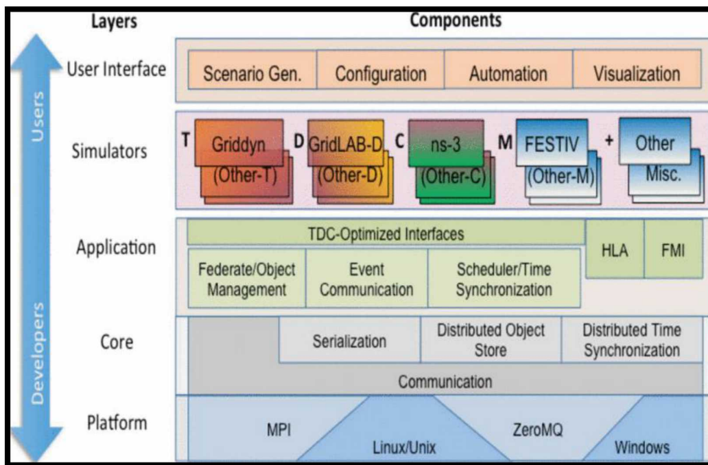
Figure 11: Architecture of the HELICS tool [20].
