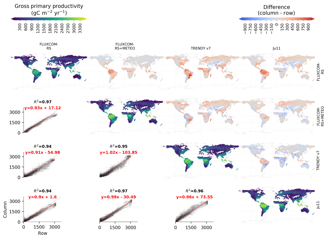
Figure 2. Comparisons of mean annual GPP at 1^\circ spatial resolution for the period 2008–2010 of FLUXCOM ensemble products with Ju11 and the mean of 16 TRENDY models. The diagonal denotes maps of mean annual GPP. Above the diagonal denotes maps of GPP differences (product along column – product along row). Below the diagonal denotes the 1 : 1 regression where the shading shows point density. The red line and equations show the best-fit line from total least-squares regression.
