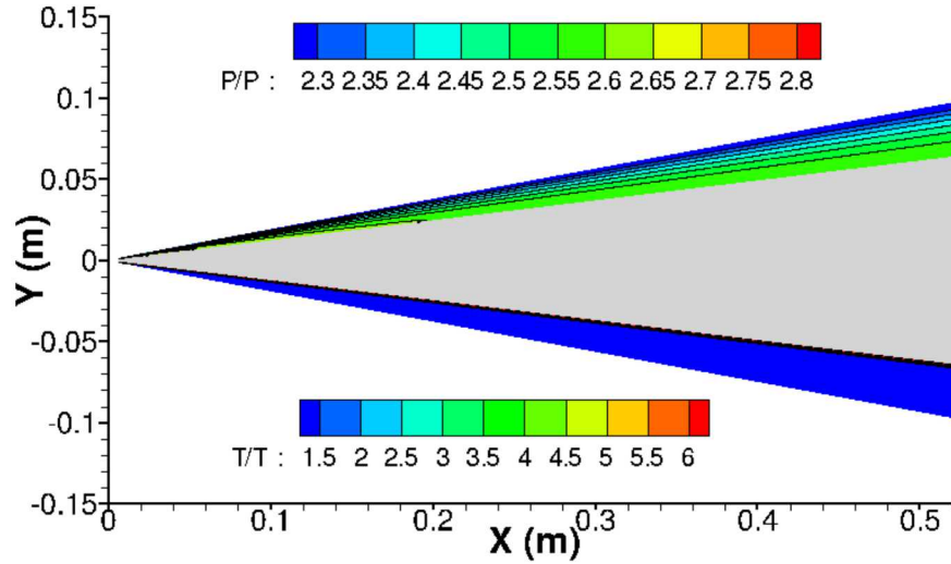
Figure 8: Meanflow pressure ratio P/P_\infty (top) and temperature ratio T/T_\infty (bottom) contours over smooth cone.
