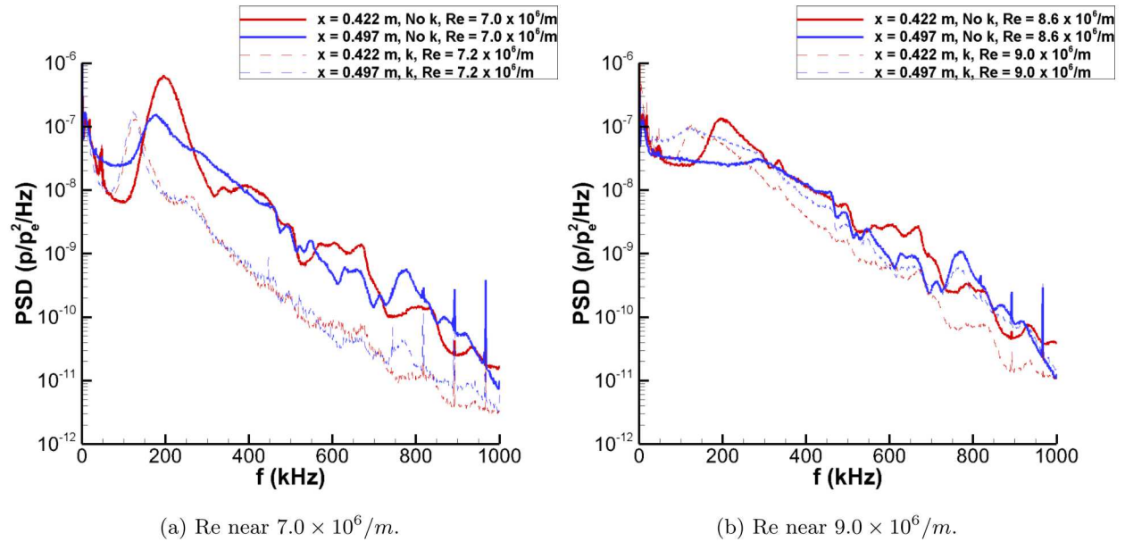
Figure 14: Mach 8: comparison of pressure spectra at x = 0.422 and 0.497 m.
