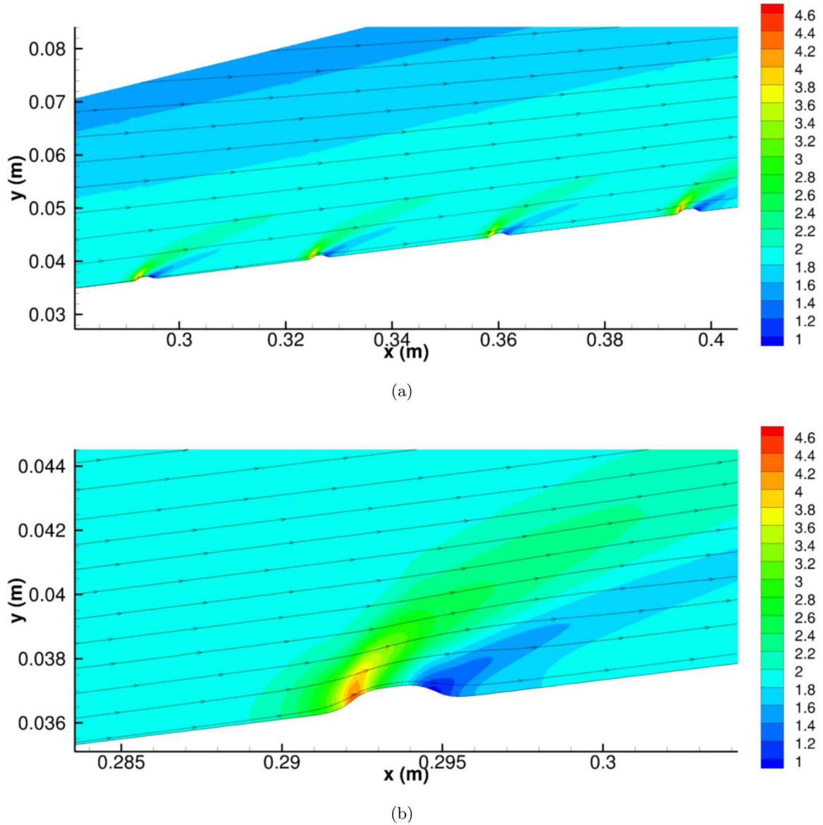
Figure 22: (a) Meanflow pressure contours, P/P_\infty , over roughness. (b) Stream trace around roughness element.
