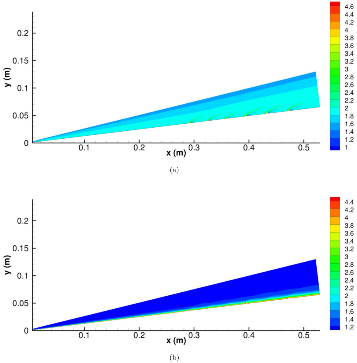
Figure 21: (a) Meanflow pressure, P/P_\infty , and (b) temperature, T/T_\infty , contours over roughness array.
