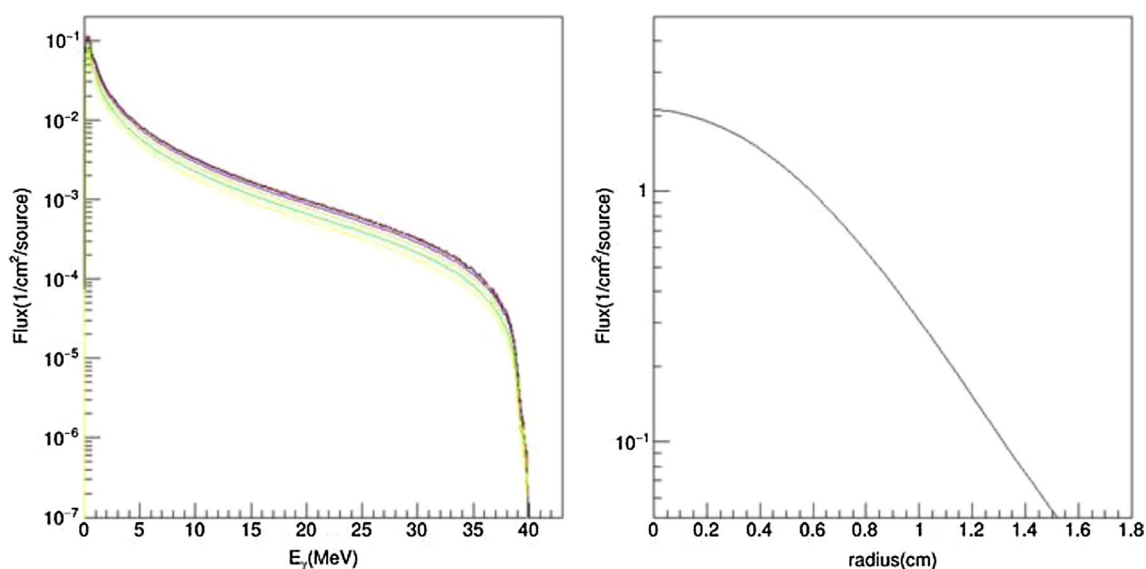
Fig. 3 Left: flux vs. energy from 0.5 mm (black—on top) to 6 mm (yellow) in radius. Right: radial dependence of photon flux in the Mo target
