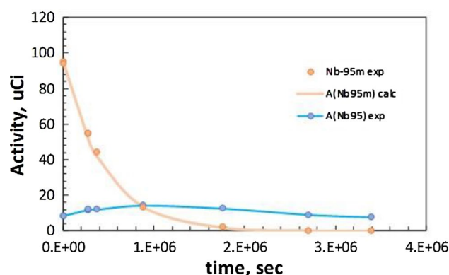
Fig. 4 Ingrowth of ^{95}\text{Nb} from decay of ^{95\text{m}}\text{Nb}
