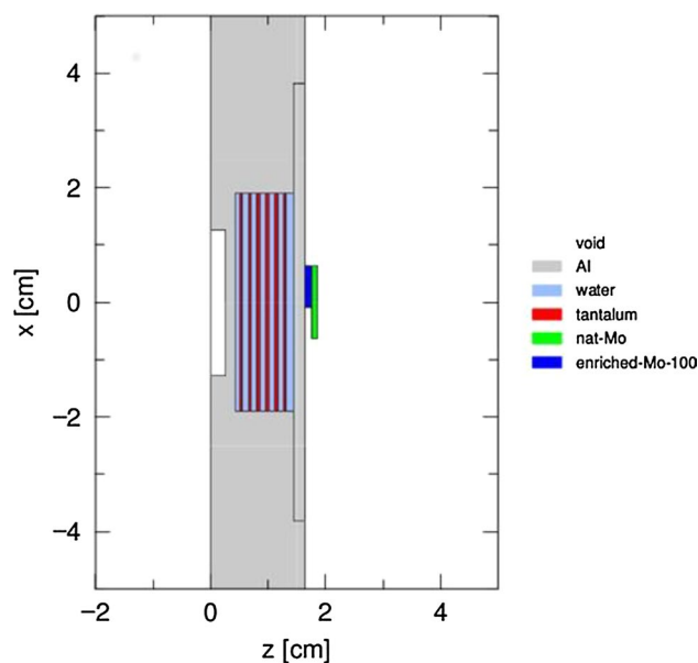
Fig. 2 Geometry of clamshell setup for natural and enriched ^{100}\text{Mo} targets
