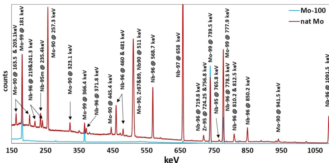
Fig. 5 Gamma spectra of irradiated natural UHP and ^{100}\text{Mo} -enriched Mo targets
