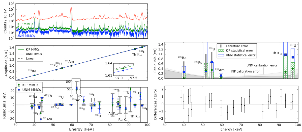
Figure 27 (left): MMC spectra (top), calibration (center) and residuals (bottom) from the same ^{233}\text{U}/^{239}\text{Pu} source, once measured with MMCs from the Heidelberg Kirchhoff Institute for Physics (“KIP MMCs”, green) and once with MMCs from STAR Cryo / U of New Mexico (“UNM MMCs”, blue). Both detectors can be calibrated with a simple second-order polynomial, and the non-linearity of the smaller UNM MMCs is larger as expected (center). The residuals for both MMCs agree for all lines within the error of the measurement, suggesting that non-zero deviations from the literature values are due to a literature error rather than detector artifacts. Figure 28 (right): The precision of the MMC measurements is comparable to the precision of the calibration lines in the literature (top). The difference between the UNM and the KIP MMCs are consistent with the error of the measurement for all lines in the spectrum, i.e. the ratio of difference / error is consistent with zero within the error bar of the measurement (bottom) [Kim 2018b].
