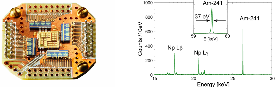
Figure 1 (left): Picture of a 32-pixel MMC \gamma -detector array (center) surrounded by four blueish SQUID preamplifier chips [Boyd 2020]. Figure 2 (right): High-resolution Am-241 \gamma -ray spectrum from a 14-pixel MMC array [Boyd 2018].
