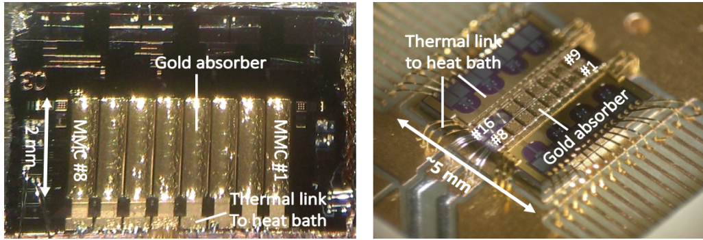
Figure 26: MMC gamma detectors developed at the Kirchhoff Institute of Physics (KIP) at Heidelberg University (left) and at the University of New Mexico (UNM) (right).
