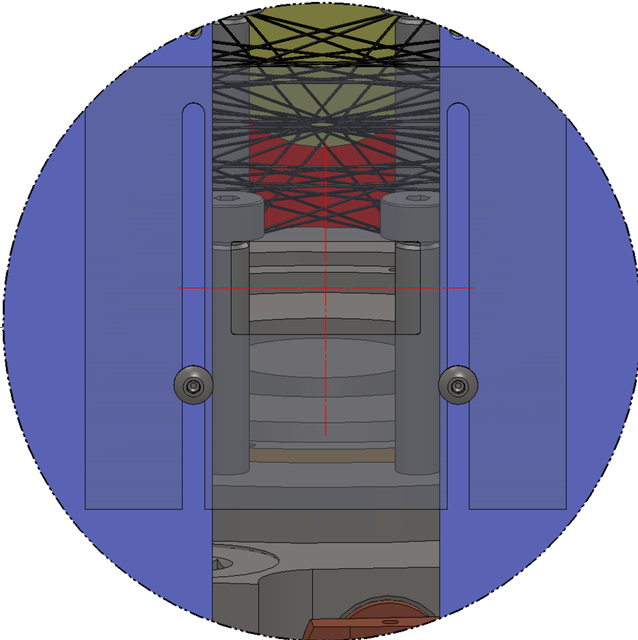
DETAIL D SCALE 4 : 1
