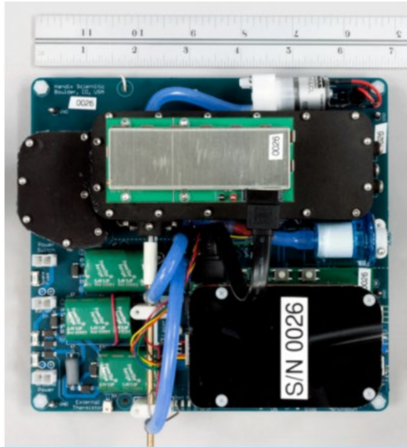
Figure 1. POPS-AIR photograph from the manufacturer's website ( http://www.handixscientific.com/pops ).
