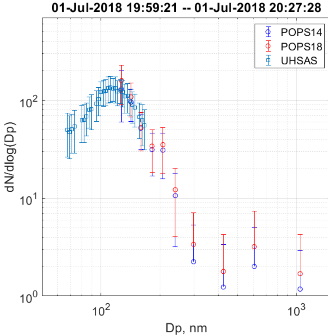
Figure 5. Comparison of the size distribution between two TBS POPS-AIR and the UHSAS from the third ARM Mobile Facility (AMF3) during the Profiling at Oliktok Point to Enhance Year of Polar Prediction (YOPP) Experiments (POPEYE) deployment in July 2018.
