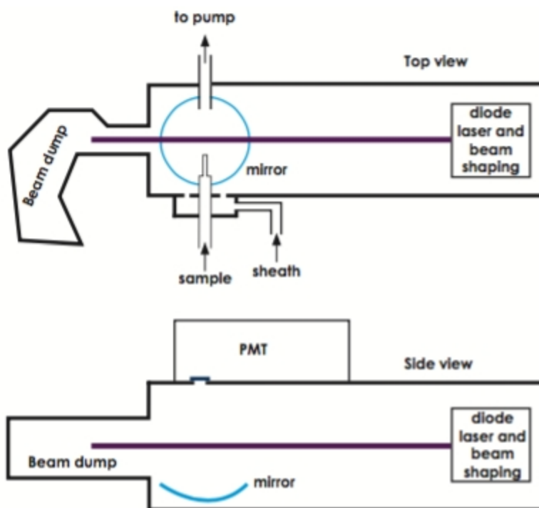
Figure 2. Schematic of POPS-AIR optical chamber, showing 405-nm laser diode and beam dump. Information from the manufacturer's website ( http://www.handixscientific.com/pops ).
