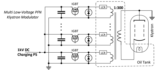
Figure 4: The configuration of NSLS-II solid-state switching klystron modulator with an array of small “PFN” modules which uses IGBT switches and operate in parallel at a much lower voltage (~1kV).
