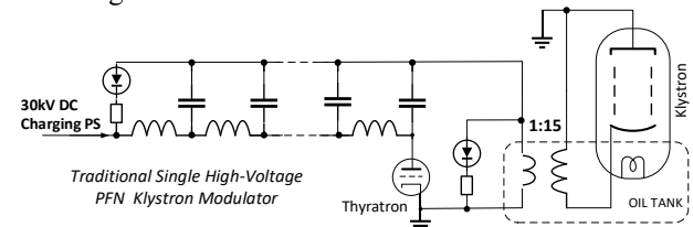
Figure 3: The traditional PFN klystron modulator with a single PFN section.
