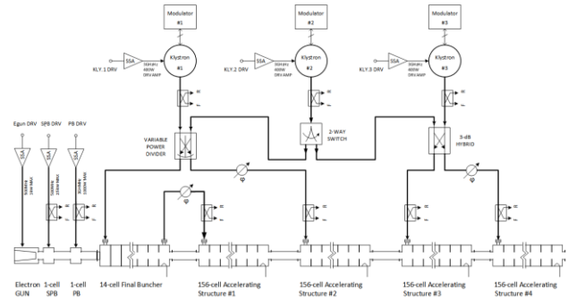
Figure 2: The NSLS-II LINAC rf power plants is comprised of three Solid-State RF PA's and three 45MW klystrons for the following 4-section 3GHz accelerating structures. The klystron in position #1 and 3 are for normal operation, while the one in #2 is a backup station.
