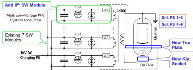
Figure 6: The necessary modification on the old K2 modulator for upgrading its capacity to support the bigger E37302A klystron.
