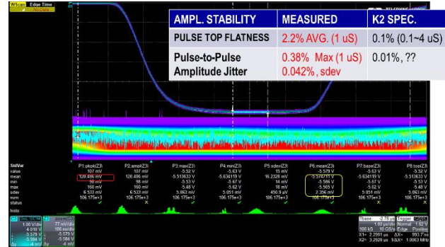
Figure 8: Amplitude stability performance of CPI-rebuilt Thales TH2100A klystron running on a ScandiNova K2 modulator.
