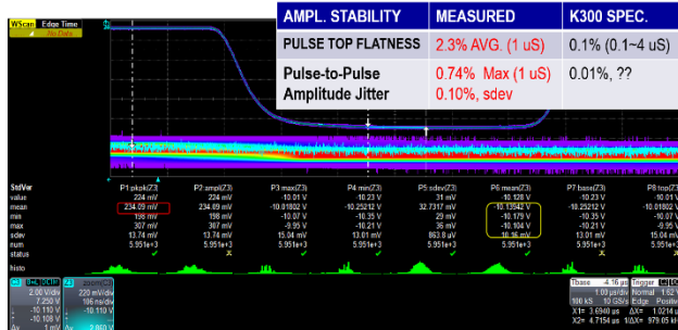
Figure 7: Measured stability performance of BNL's first K300 modulator running with a E37302A klystron.
