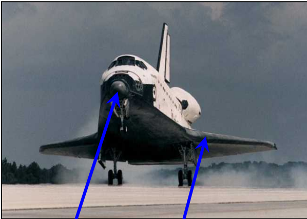
Wing Leading Edge & Nose Cap RCC Panels
