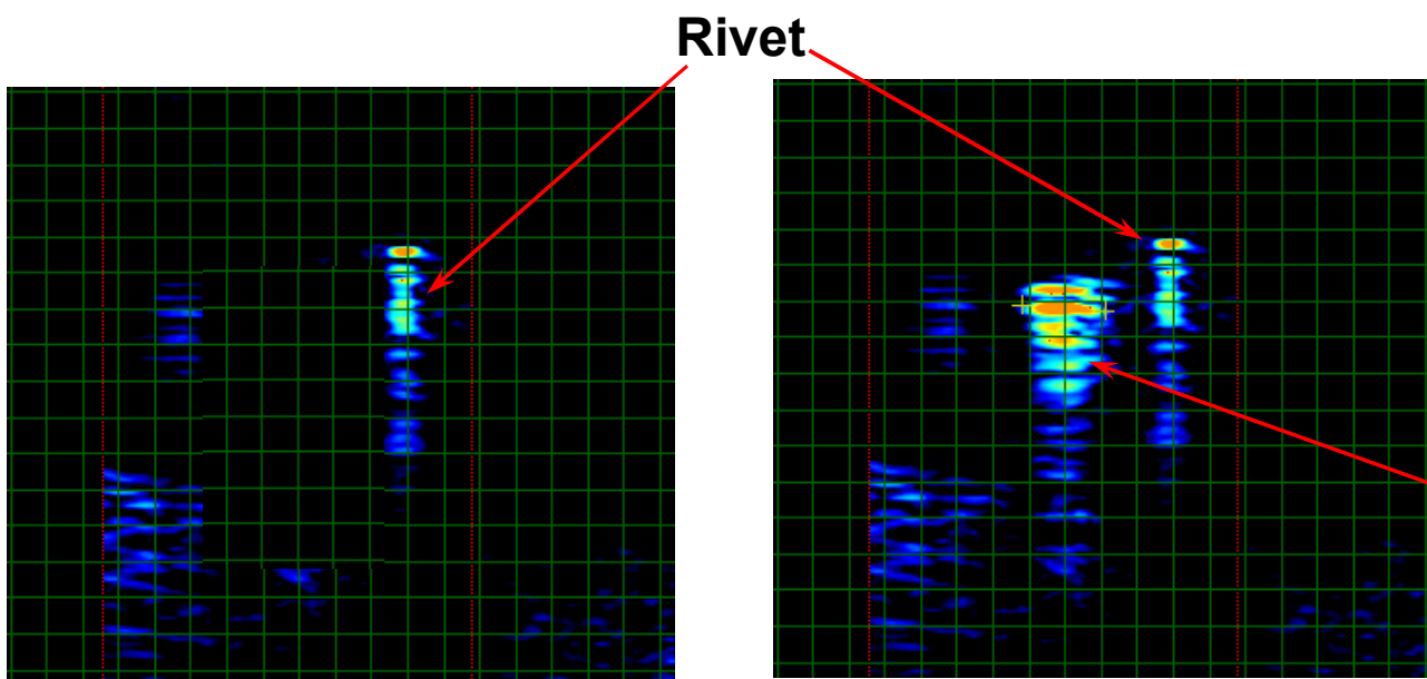
Rivet with crack
