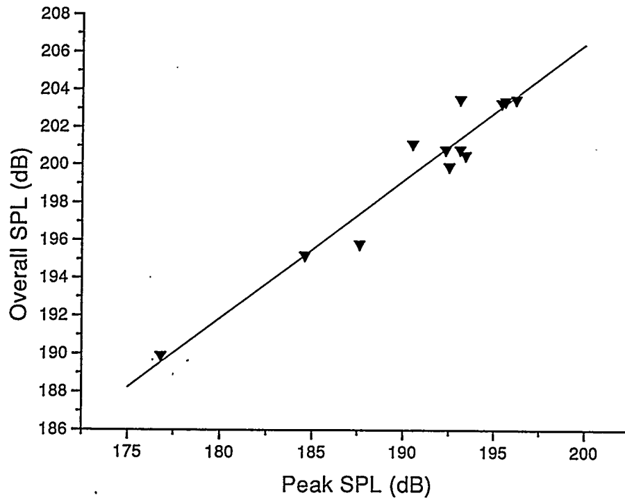
Figure 37. Relationship Between Peak and Overall Sound Pressure Levels
