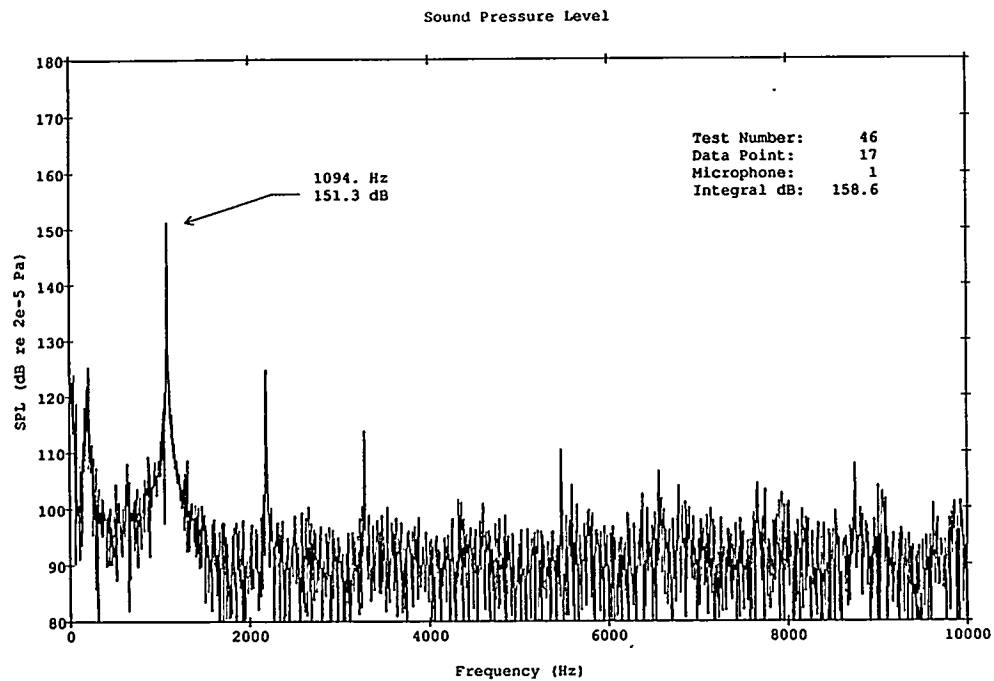
Figure 24. Sound Pressure Level vs. Frequency with 1000 Hz Pulse Combustor Tuned In.
