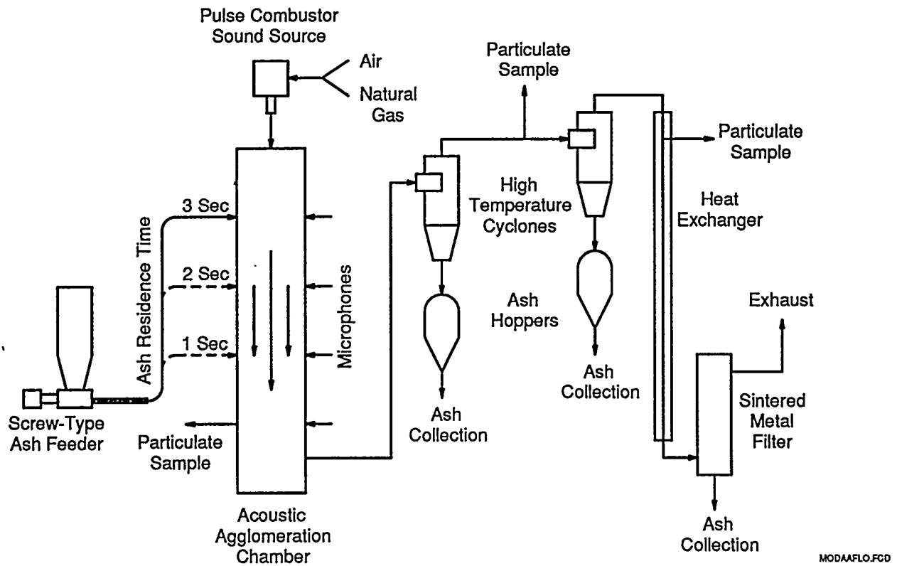
Figure 2. Low Frequency Agglomeration Flow Diagram
