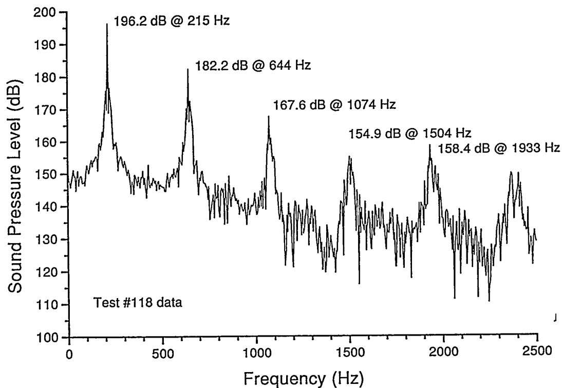
Figure 36. Harmonic Sound Pressure Level Peaks
