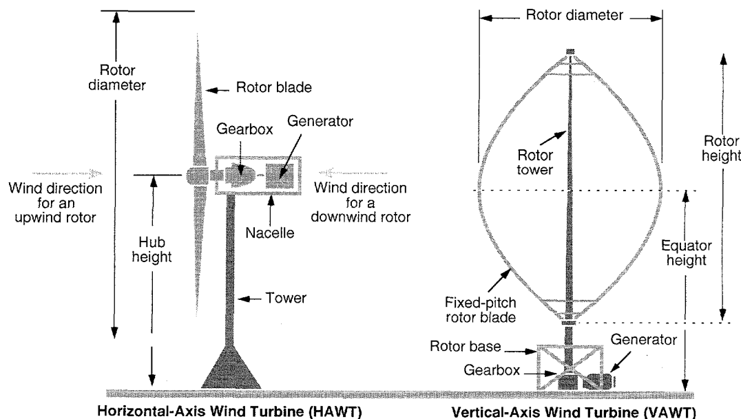
Figure 22. Wind Turbine Configurations
