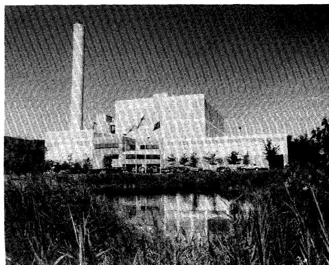
The Bristol Resource Recovery Facility, which began commercial operation in May 1968, converts up to 650 tons of solid waste to saleable energy each day. At maximum output, the plant generates over 16 megawatts; remaining electricity is sold to a local utility and used to power area homes and businesses. (Source: Ogden Martin Systems of Bristol, Inc.)
