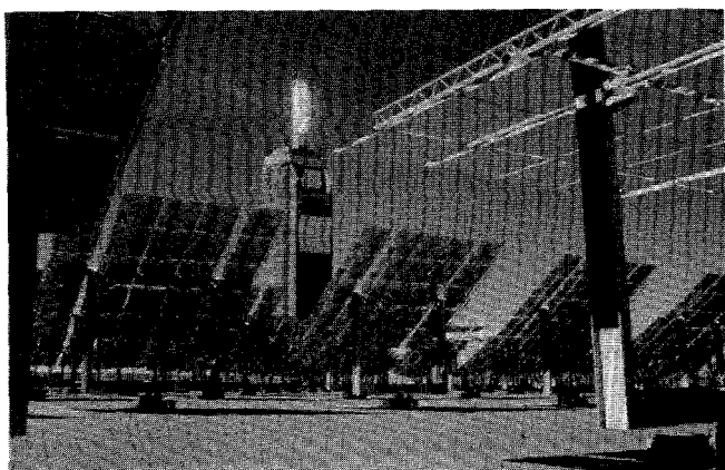
Central receiver power plant at Sandia National Laboratory in Albuquerque, New Mexico. The plant consists of a large central tower, which houses the receiver, and a surrounding field of heliostats. The heliostats are large mirrors mounted on moveable frames that can track the sun and concentrate the sunlight onto a specific point, the receiver, on the tower. Inside the receiver, a pressurized fluid will be heated by the concentrated sunlight, become a gas, and drive a generator to produce electricity.
