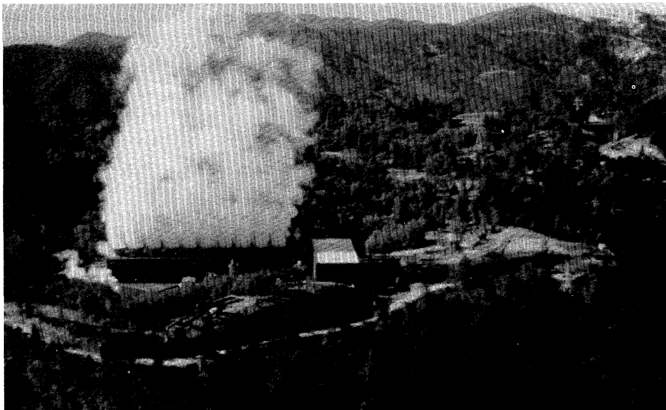
Overview of The Geysers, Unit 13, a 135-megawatt power plant with Stretford primary abatement system.
