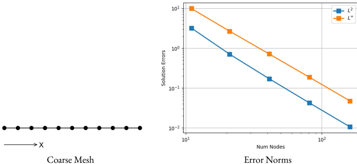
Figure 3.8-2.. Transient Heat Conduction: 3D Bar2 Meshes
