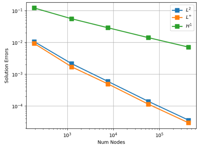
Error Norms
