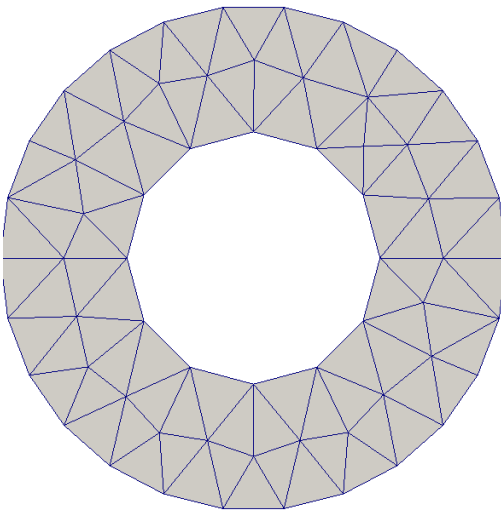
Coarse Mesh
