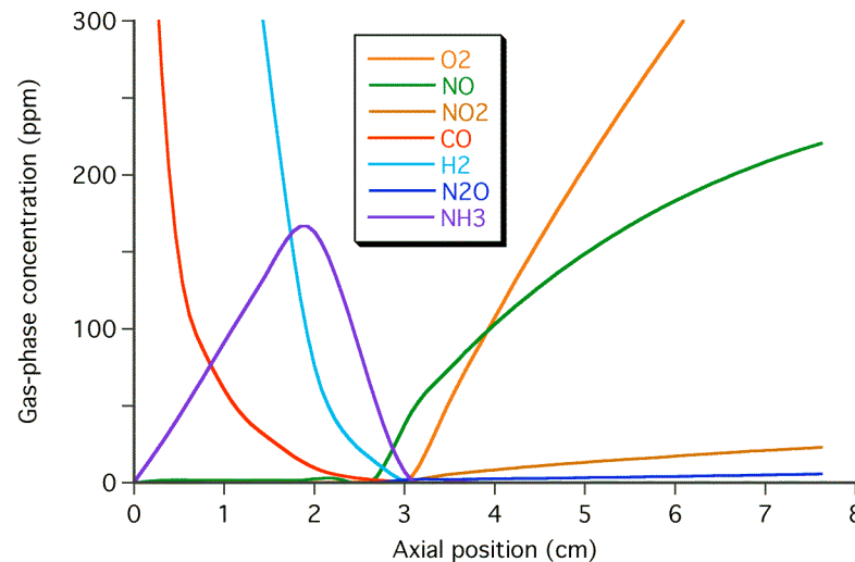
Axial profiles of gas-phase species concentrations at 923 s during long storage/regeneration cycle at 400 C
