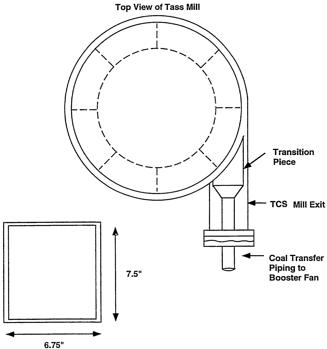
End View of Mill Exit Prior to Installing Transition Piece
