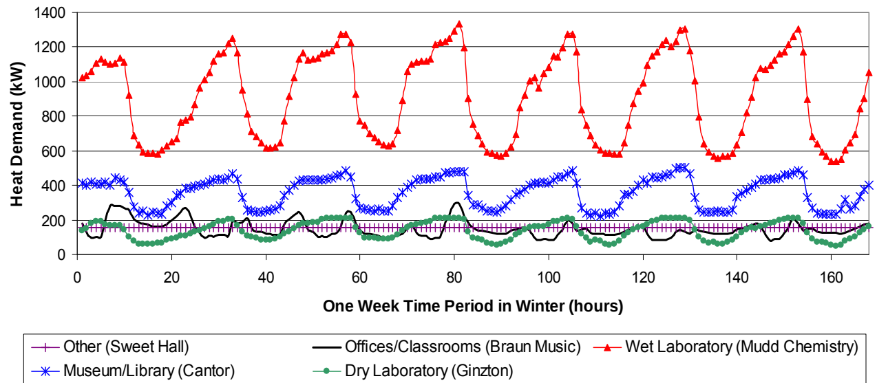
Heating Demand over One Week in Winter for Five Buildings
