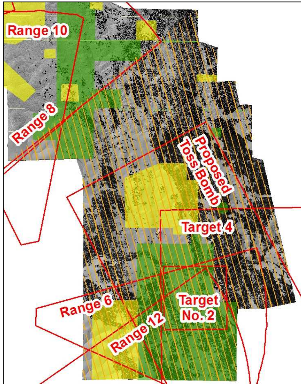
Figure 10. The 81-mm mortar transect design (orange lines) overlaid on a shaded relief of the lidar data for the southern part of Camp Beale. The ranges associated with the identified targets are outlined in red and labeled. The yellow and green regions are areas that show munition-related features based on the lidar data.
