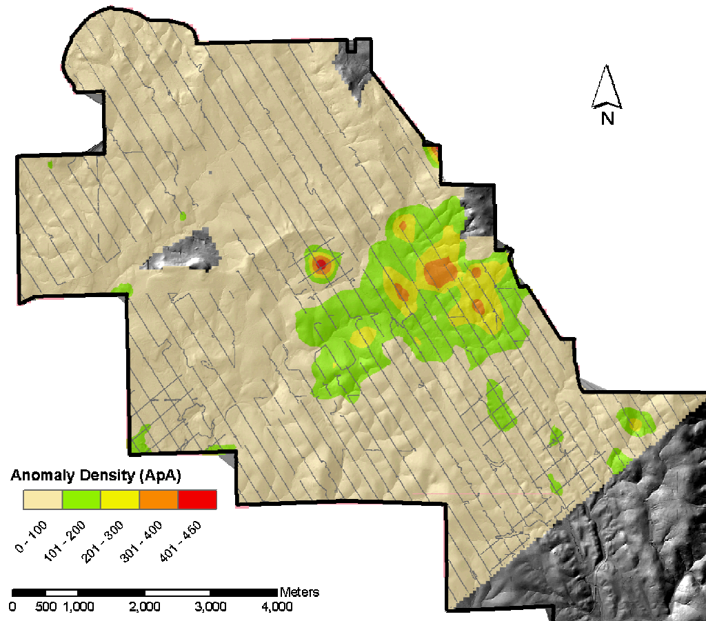
Figure 27. Anomaly density values (ApAs) for the 100-lb bomb and 105-mm projectile combined analysis area. Areas without color shading were not estimated because no observational data were available. Gray-colored lines show transect sample locations.
