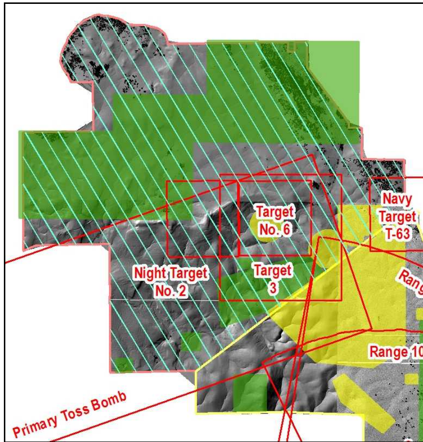
Figure 6. The 100-lb bomb transect design (blue lines) overlaid on a shaded relief of the lidar data for the northern area of Camp Beale. The five ranges associated with the identified targets are outlined in red and labeled. The yellow regions are those areas that show munition-related features based on the lidar data and the green regions show man made features that may be munitions related.
